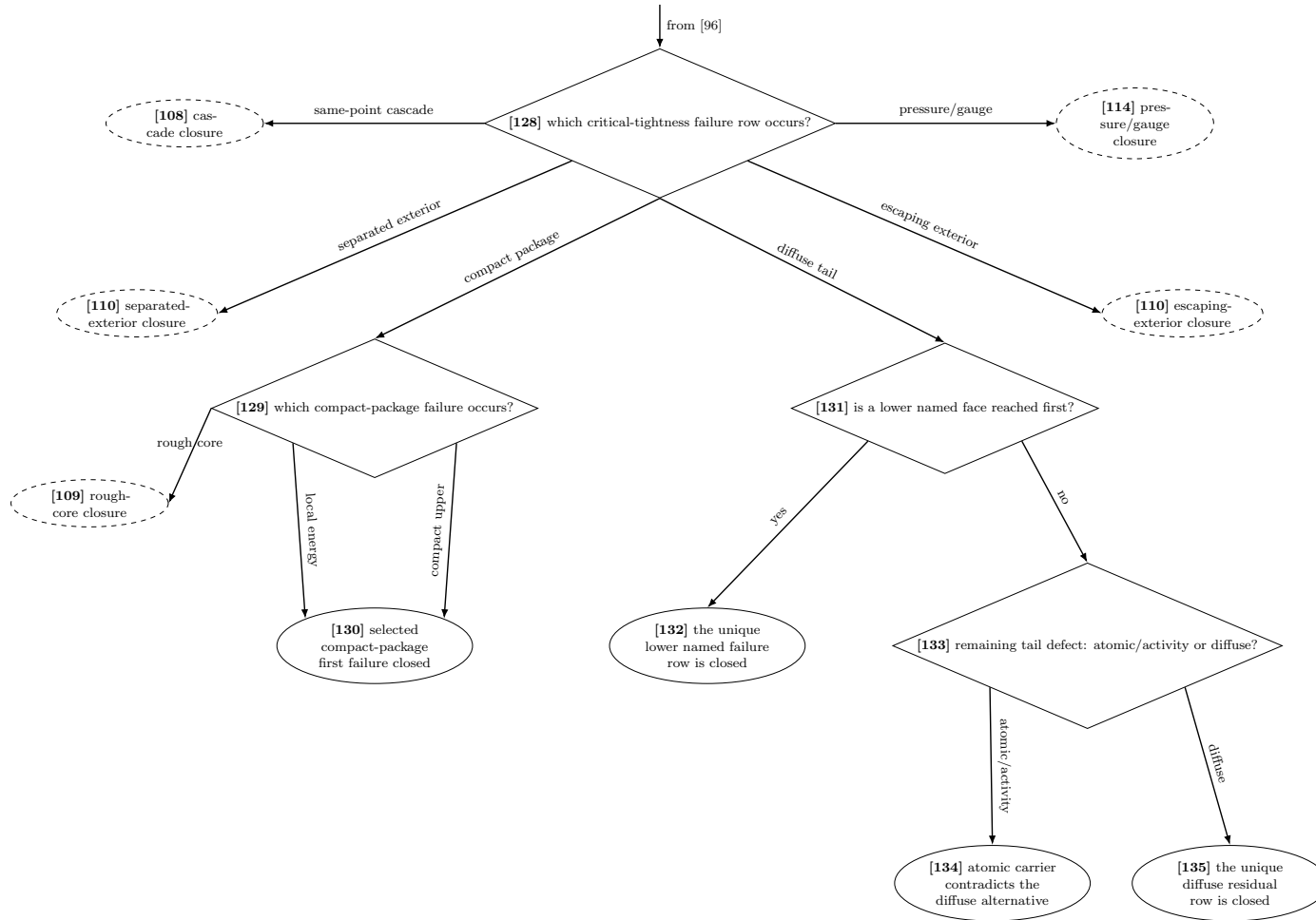
FIGURE 12. Proof-dependency diagram, Part XII. The six alternatives of lemma 10.102 leave [128] on separate edges. The compact-package and diffuse-tail cases are further split at [129] and [131]. The proof of lemma 10.103 tests for a lower named face first, then applies the atomic/diffuse dichotomy at [133]. Dashed ellipses refer to terminal closures already drawn in Parts IX–XI.
