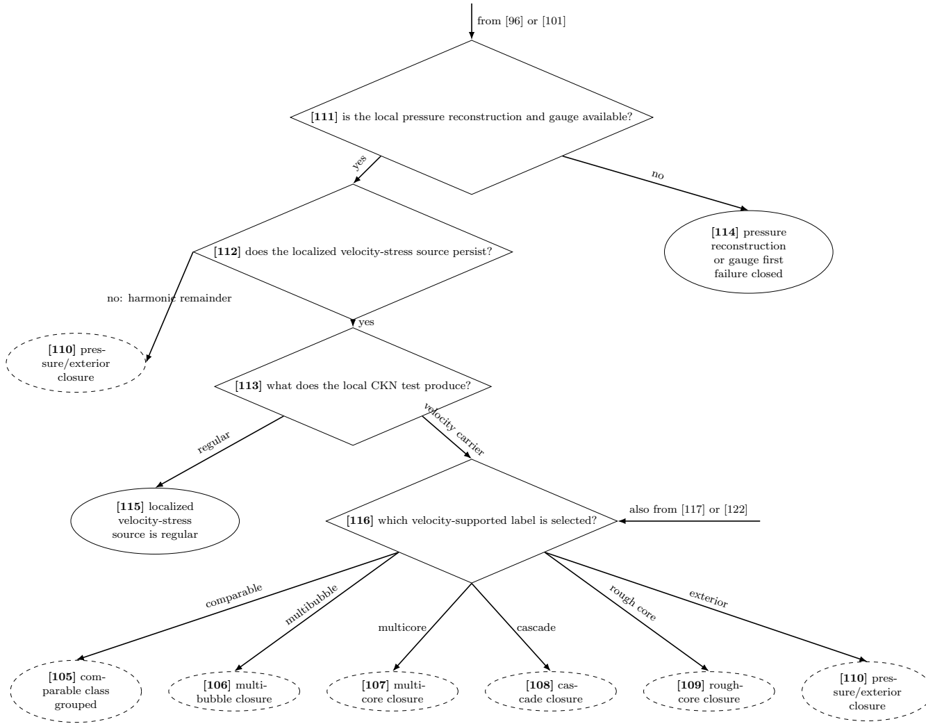
FIGURE 10. Proof-dependency diagram, Part X. The proof of lemma 11.32 first tests the pressure reconstruction at [111], then the localized source at [112], and only then runs the local CKN test [113]. A velocity carrier is classified at [116], which also receives the velocity-supported outcomes of [117] and [122]. Dashed ellipses are references to terminal closures proved and drawn as solid ellipses in Part IX.
