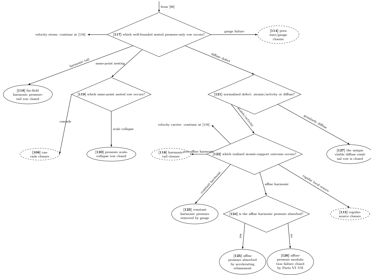
FIGURE 11. Proof-dependency diagram, Part XI. The five rows of lemma 9.67 are explicit at [117]. The same-point row splits at [119]. The proof of lemma 9.68 first makes the atomic/diffuse test [121], then classifies a realized atomic support profile at [122]. Dashed ellipses refer directly to terminal closures drawn elsewhere.
