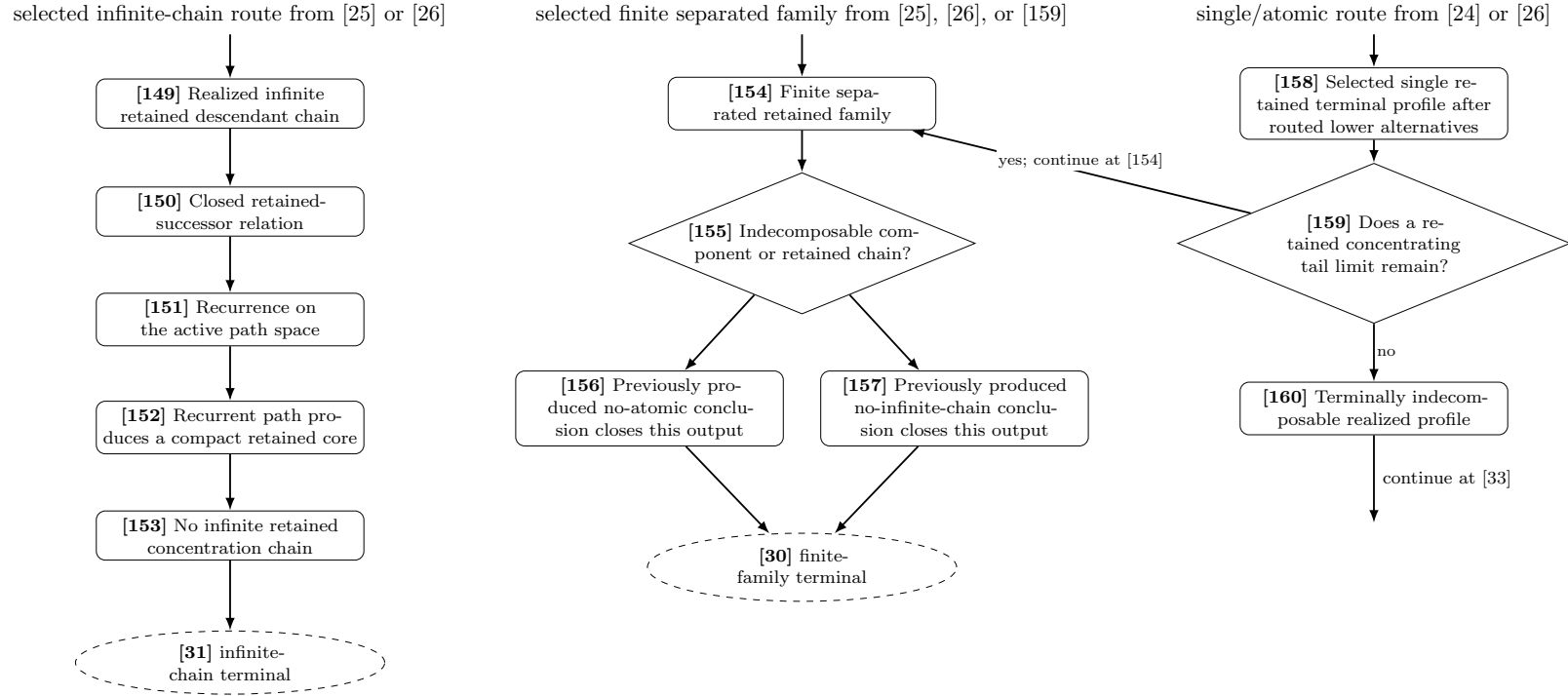
FIGURE 12. Proof flow, Part XII: recurrence, finite separated-family exclusion, and production of the terminally indecomposable input. Sequence- L^3 and mildness are still downstream: they are produced at [34] and [36] only after the route reaches [33].
