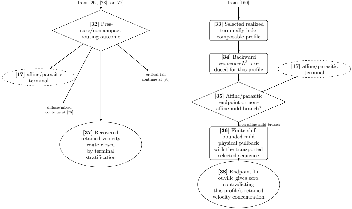
FIGURE 4. Proof flow, Part IV: chartwise pressure routing and endpoint input production. Sequence- L^3 is produced at node [34], and finite-shift mildness is produced only on the non-affine branch at node [36]. The terminal theorem and the final residual/setup assemblies are downstream consumers of the displayed branch closures.
