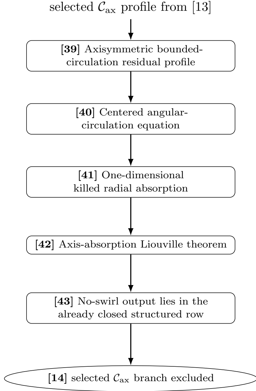
FIGURE 5. Proof flow, Part V: the complete axisymmetric bounded-circulation closure. The terminal at [14] is reached only after the circulation equation, absorption lemma, and no-swirl routing have been produced.
