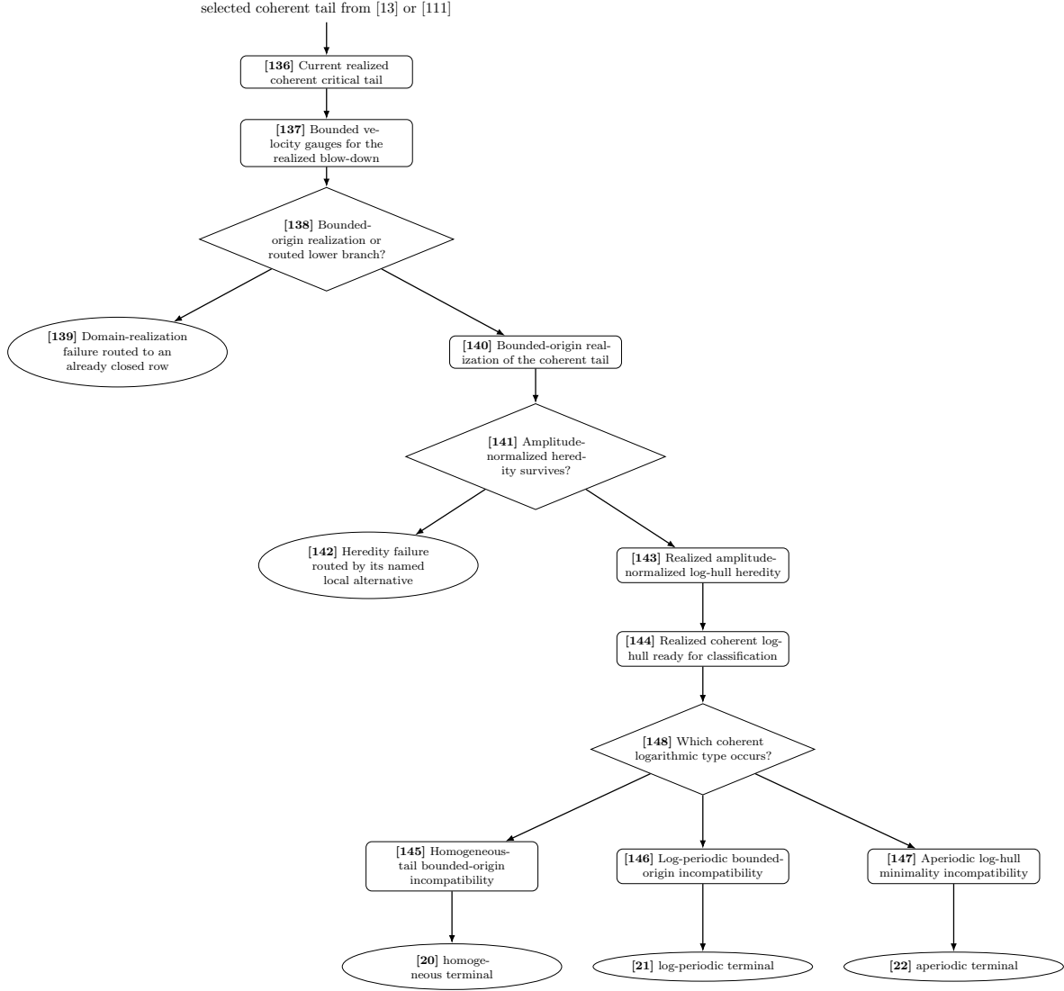
FIGURE 11. Proof flow, Part XI: bounded-origin realization and the three coherent critical-tail closures. The homogeneous, log-periodic, and aperiodic outputs remain distinct through their terminal contradictions.
