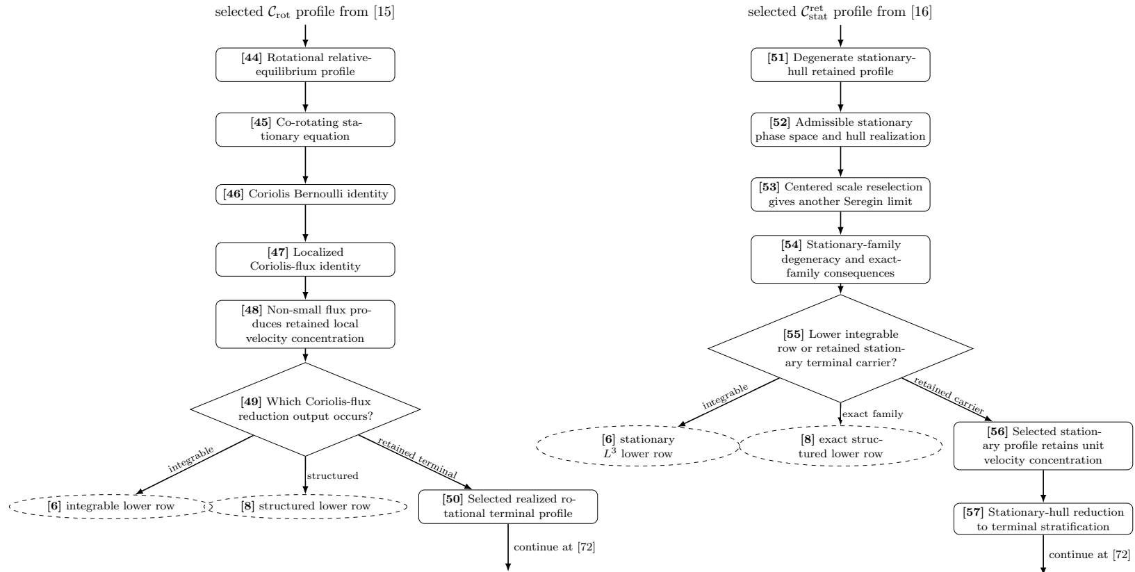
FIGURE 6. Proof flow, Part VI: the internal R2 and R3 reductions. Neither row receives sequence- L^3 as an entry hypothesis. Each retained output continues to the common selected terminal-recentering protocol at [72].
