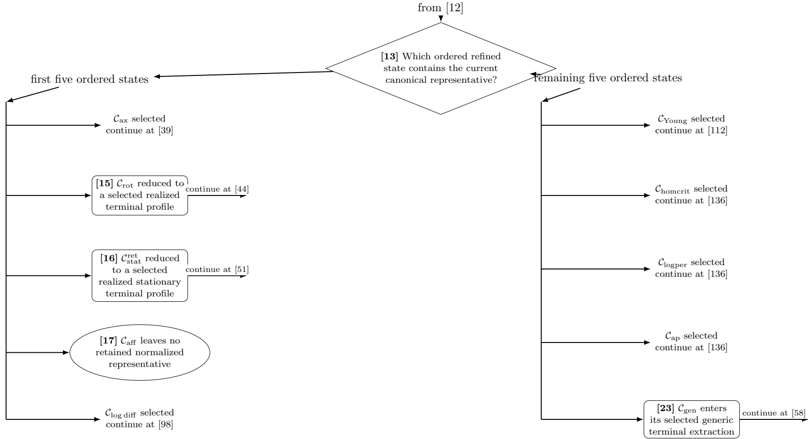
FIGURE 2. Proof flow, Part II: the complete ordered refined selection at node [13]. The two unnumbered headings only distribute the ten outgoing cases for readability. They do not introduce states or hypotheses. Every unfinished selection continues to its displayed local module.
