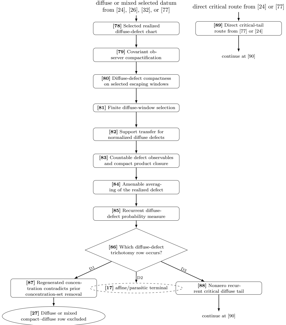
FIGURE 8. Proof flow, Part VIII: diffuse-defect compactification and the exact D1–D3 trichotomy. Regenerated concentration, affine collapse, and a critical diffuse tail are displayed separately.
