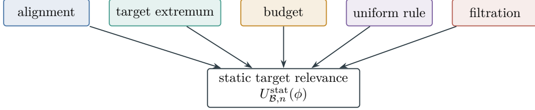
Figure 6: Static target relevance is a same-observable conjunction. Target separation and extremum consistency are combined with a charged construction, one family rule, and a monotone terminal filtration; failure of any gate sets the product in Definition I.4.3 to zero.
