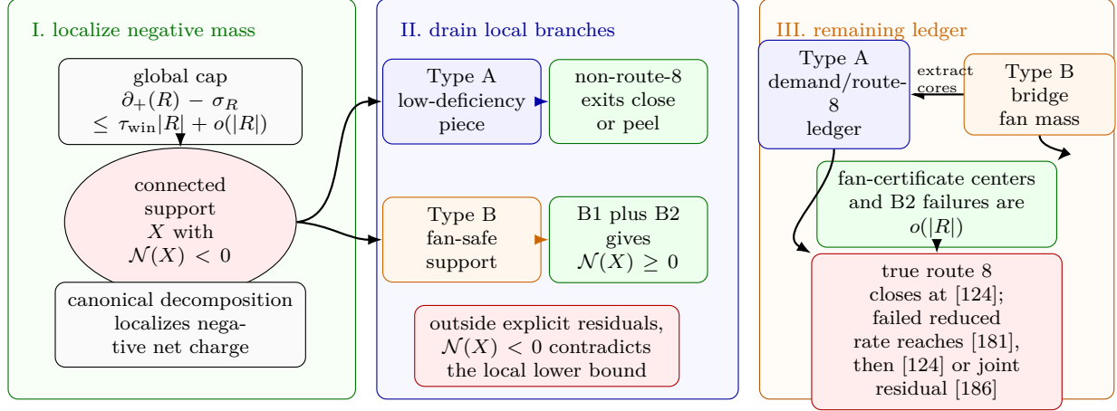
Figure 32: Visual proof of the branch-reduction mass ledger. Panel I shows the large-budget cap localizing negative net charge to a connected admissible support X with \mathcal{N}(X) < 0 . Panel II shows the local branch drain used in Theorem 15.1 : Type A supports close through the non-route-8 exits or enter target-defect peeling, while Type B supports close through the B1 ledger together with B2, giving \mathcal{N}(X) \geq 0 outside the explicit residuals. Panel III records the remaining global ledger. Type B bridge and fan-mass residuals are charged to assigned surplus units and become o(|R|) after route-8 non-window cores are extracted into the Type A ledger. The unified demand ledger counts both target-defect and route-8 Type A entries. Target-defect two-support entries are canonical exit-(4) peel data, and every peel remains charged by the exact stage accounting. A true two-support route-8 terminal is excluded at node [124]; failure of the reduced-stage rate reaches the peeled-demand ledger at [181], whose maximal-ledger augmentation routes the witness-free arm to [124]. On the surviving [183] arm, shortest-trace boundary-support exhaustion proves the silent entry count zero and reaches [184]. On [184], visible-first prefix exhaustion proves the non-overloaded count zero and canonically packages four actual visible returns at every entry receiver, reaching [185]. The simultaneous account at [185] then proves every saturated routed load visible and appends the coupled peel, deficit, demand, absorption, and open-unit balances at [186].
