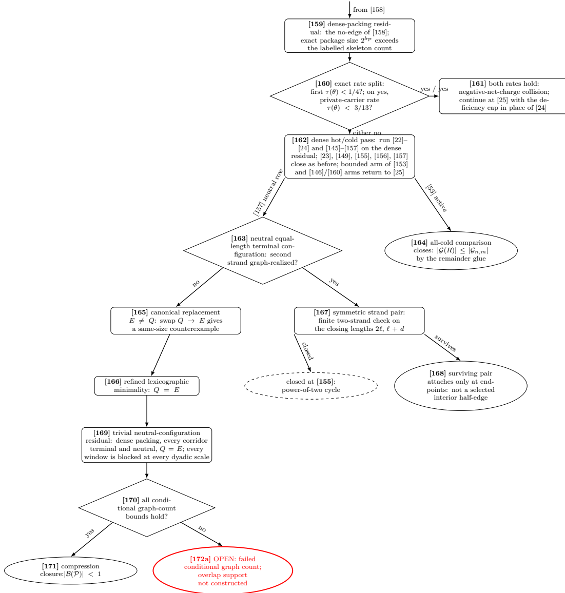
Figure 12: Proof-dependency diagram, Part XII. The dense residual [159] passes through the two exact rate tests at [160]. Only the arm satisfying both the net-deficiency rate \tau(\theta) < 1/4 and the route-8 private-carrier rate \tau(\theta) < 3/13 enters [161]. Failure of either comparison enters the dense hot/cold pass [162] on its literal residual. The all-cold arm closes at [164]; the neutral arm [163] splits into the replacement route [165]–[166] and the two-strand route [167], [155], [168]. The dashed ellipse names the already drawn closure [155]. The trivial neutral residual [169] reaches the proved closure [171] through the positive decision at [170], carrying both the graph-count inequalities and the exact overflow from [159]. The negative arm retains the first failed conditional graph-count inequality, its outside record and prefix, and every inherited fact, and stops at the open leaf [172a]. At the selected graph the positive decision is empty ( Corollary 7.44 ): the aggregate inequalities hold only for an empty blocked class, so every selected graph reaching [169] stops at [172a]. No overlap support or serial system has been constructed from that failure, and no exact-lift or full-state step follows [172a] in the proof graph.
