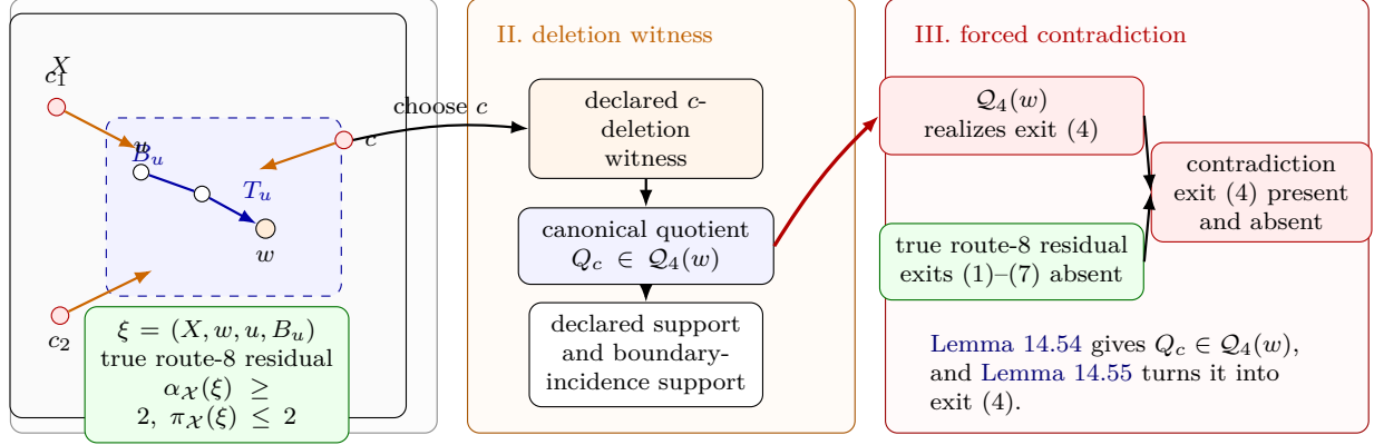
Figure 26: Visual proof of the terminal two-support route-8 exclusion. Panel I shows a terminal entry \xi = (X, w, u, B_u) . The grey rectangle is the Type A support X , the blue dashed region is the target-complete-minimal basin B_u , the orange vertex is the saturated receiver w , and the red boundary nodes are essential boundary incidences. The displayed terminal data are \alpha_X(\xi) \geq 2 , \pi_X(\xi) \leq 2 , and true route-8 residuality. Panel II isolates one essential incidence c . Its declared deletion witness has declared support and boundary-incidence support, and the two-support deletion lemma places the corresponding quotient in the canonical exit-(4) family \mathcal{Q}_4(w) . Panel III records the contradiction: the response-support deletion-exit lemma realizes exit (4) at w , while true route-8 residuality says that exits (1)–(7), including exit (4), are absent. Thus the terminal two-support obstruction of Definition 14.60 cannot occur.
