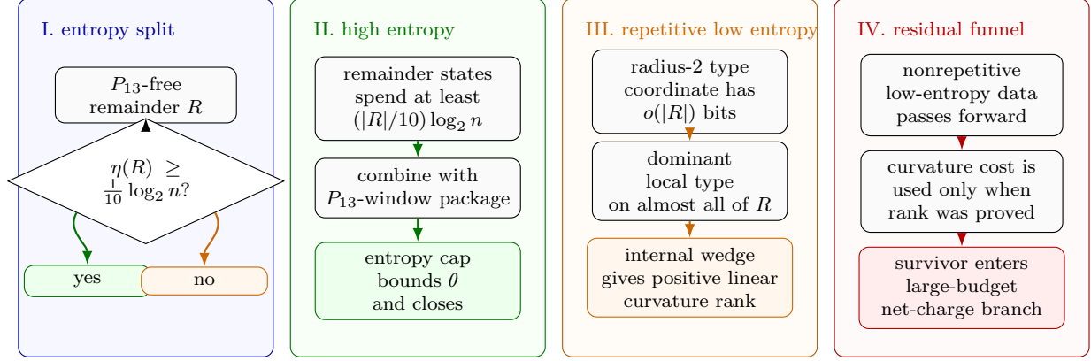
Figure 19: Visual proof of the two-budget routing funnel. Panel I splits the P_{13} -free remainder by its per-vertex skeleton entropy \eta(R) . Panel II shows the high-entropy branch: \eta(R) \geq \frac{1}{10} \log_2 n spends (|R|/10) \log_2 n bits, and together with the independent P_{13} -window package gives the packing bound used by the entropy cap. Panel III shows the structurally repetitive low-entropy branch: subexponential radius-2 type data gives a dominant local type, and an internal length-two wedge in that type supplies positive linear curvature rank. Panel IV records the routing convention of Proposition 11.6 : nonrepetitive low-entropy data is passed to the large-budget net-charge branch, and curvature cost is carried forward only on branches where the preceding rank-forcing lemmas have established it.
