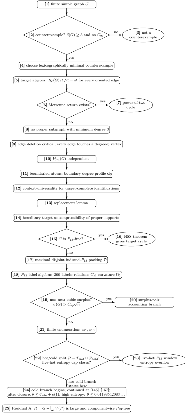
Figure 1: Proof-dependency diagram, Part I. Rectangles are assertions or residual states, diamonds are yes/no branch tests, ellipses are terminal outcomes, and edge labels such as yes or no state which branch is followed. The bracketed numbers are unique diagram-node numbers used by the dependency table. Nodes [19] and [20] record the non-near-cubic surplus accounting branch used before the normalized spine budget; node [20] is the continuation expanded in Fig. 10. Node [22] creates the hot/cold dichotomy by splitting \mathcal{P} into \mathcal{P}_{\text{hot}} and \mathcal{P}_{\text{cold}} . Its no-branch is the start of the cold branch, recorded at [24] and expanded at [145]–[157] in Fig. 11. Node [25] continues in Fig. 2.
