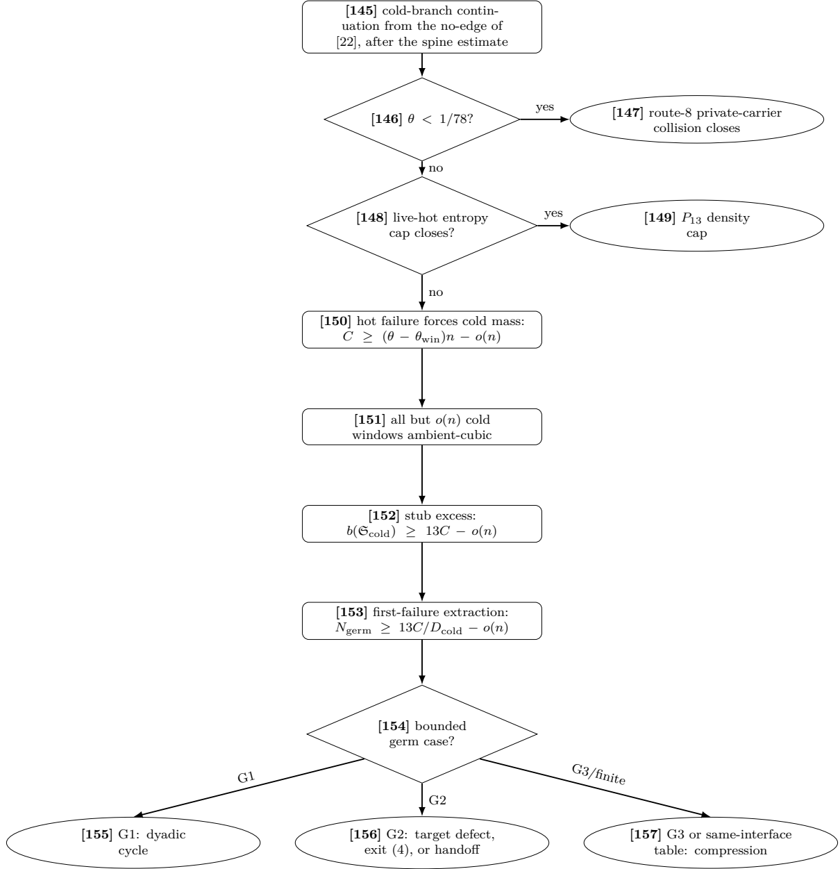
Figure 11: Proof-dependency diagram, Part XI. This panel continues the cold branch that begins on the no-edge of the hot/cold split at node [22] and is recorded at node [24]. Node [22], rather than this panel, creates the dichotomy \mathcal{P} = \mathcal{P}_{\text{hot}} \sqcup \mathcal{P}_{\text{cold}} . If \theta < 1/78 , the existing route-8 carrier inequality closes at [147]. Otherwise the live-hot entropy cap either yields the density cap [149], or its failure forces the unpaid cold family to have linear size [150]. On the near-cubic spine, only o(n) cold windows are non-cubic [151]; each ambient-cubic cold window has 15 external stubs, and after two corridor ends are absorbed it contributes 13 branch-excess units [152]. The first-failure extraction [153] assigns those selected half-edges to bounded cold germs and then uses the bounded-overlap constant D_{\text{cold}} to obtain a linear disjoint family. The germ trichotomy [154] has no terminal residual: G1 gives a dyadic cycle [155], G2 routes to target defect, exit (4), or the already existing handoff ledgers [156], and G3 together with the finite same-interface table gives a target-complete compression [157].
