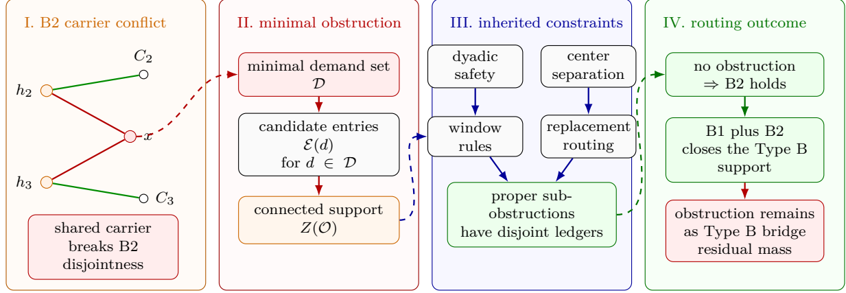
Figure 27: Visual proof of the Type B overlap-obstruction routing. Panel I shows the B2 failure mechanism: two Type B fan demands may have local B1 entries, but their candidate carrier sets can compete for a shared carrier x , so the chosen entries are not disjoint. Panel II records the finite minimality step of Lemma 14.87 : among all failed demand families, a minimal one gives a Type B overlap obstruction \mathcal{O} = (\mathcal{D}, \{\mathcal{E}(d)\}) , and its involved fan centers, carriers, paths, and window segments form the connected overlap support Z(\mathcal{O}) . Panel III displays the global constraints inherited by Z(\mathcal{O}) in Lemma 14.88 : contextual dyadic safety, high-degree separation, window compatibility, replacement/delocalization routing, and minimality of the overlap. Panel IV gives the routing consequence of Proposition 14.89 : if no such obstruction remains, B2 holds and B1 closes the Type B support; if the obstruction remains, it is a controlled Type B bridge residual charged later in the fan-mass ledger.
