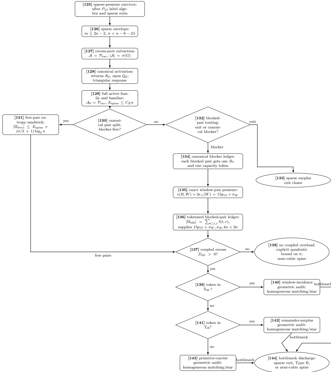
Figure 10: Proof-dependency diagram, Part X. This panel expands the sparse non-near-cubic branch [20]. Nodes [126]–[129] build the full active surplus family. Node [130] splits canonical pairs. Free pairs are charged by the entropy sandwich [131], while blocked pairs pass through the blocker route [132]–[136]; the role fibres in [136] partition \Pi_{\text{blk}} , so this ledger has no double counting. Node [137] is the coupled single-graph test of Corollaries 3.53 and 3.54 and Proposition 3.55 : all three token classes use the same n, p_{13}, \sigma_W, \sigma_R . If D_{\text{all}} = 0 , the explicit quadratic bound routes to [138]. If D_{\text{all}} > 0 , the role-fibre excess enters the window-incidence, remainder-surplus, or primitive-carrier geometric audit [140], [142], [143]. Node [144] applies Theorem 3.73 : the bottleneck realizes a sparse surplus exit, produces Type B fan data, or is bounded by fixed homogeneous caps and routes to [138].
