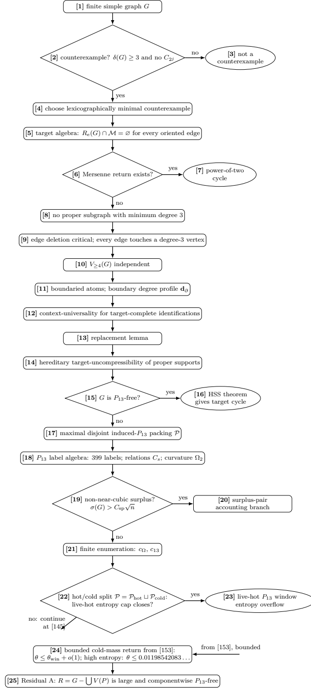
Figure 1: Proof-dependency diagram, Part I. Rectangles are assertions or residual states, diamonds are exhaustive branch tests, ellipses are terminal outcomes, and edge labels state which branch is followed. The bracketed numbers are unique diagram-node numbers used by the dependency table. Nodes [19] and [20] record the non-near-cubic surplus accounting branch used before the normalized spine budget; node [20] is the continuation expanded in Fig. 10. Node [22] creates the hot/cold dichotomy by splitting \mathcal{P} into \mathcal{P}_{\text{hot}} and \mathcal{P}_{\text{cold}} . Its no-branch continues at [145] in Fig. 11. The bounded arm of [153] returns to [24] with the density cap, and only that live residual continues to [25] and Fig. 2.
