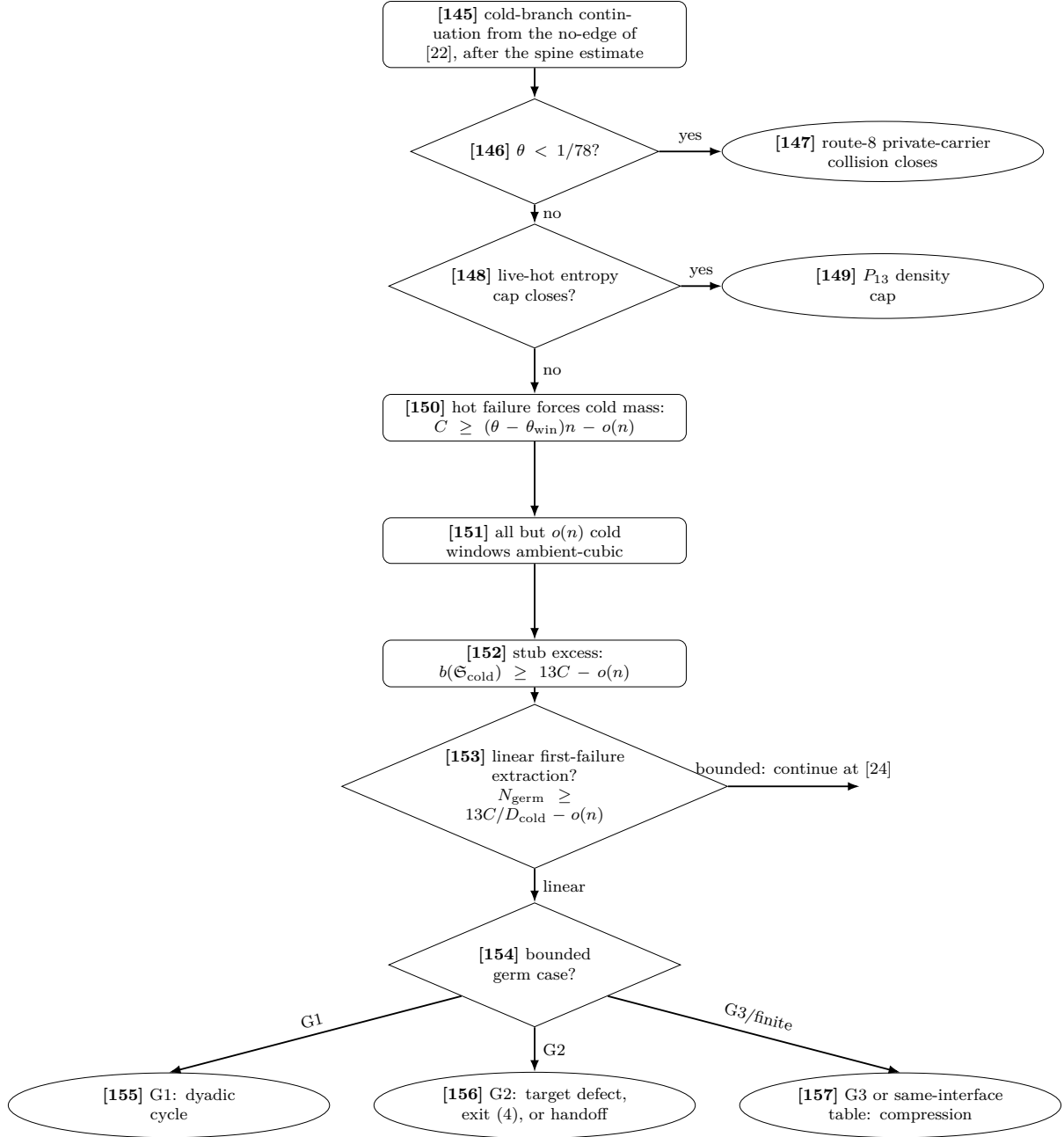
Figure 11: Proof-dependency diagram, Part XI. This panel continues the no-edge of the hot/cold split at node [22]. If \theta < 1/78 , the existing route-8 carrier inequality closes at [147]. Otherwise the live-hot entropy comparison either closes at [149], or its failure forces the unpaid cold family to have linear size [150]. On the near-cubic spine, only o(n) cold windows are non-cubic [151]; each ambient-cubic cold window has 15 external stubs, and after two corridor ends are absorbed it contributes 13 branch-excess units [152]. Node [153] makes the exact finite split hidden by the asymptotic notation: its bounded arm supplies the density cap and returns to [24], while its linear arm extracts a positive disjoint germ family and continues to [154]. The germ trichotomy [154] has no terminal residual: G1 gives a dyadic cycle [155], G2 routes to target defect, exit (4), or the already existing handoff ledgers [156], and G3 together with the finite same-interface table gives a target-complete compression [157].
