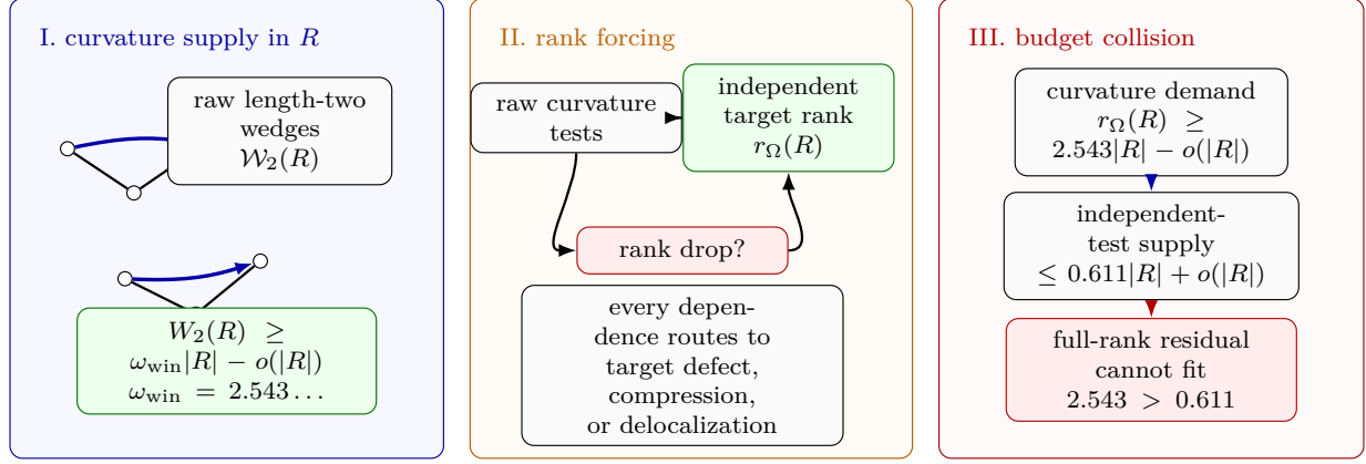
Figure 19: Visual proof of the curvature supply–budget squeeze. Panel I shows the P_{13} -free remainder R producing raw internal length-two wedge tests; the wedge lower bound gives W_2(R) \geq \omega_{\text{win}}|R| - o(|R|) , with \omega_{\text{win}} = 2.543\dots on the window-only branch. Panel II shows the rank-forcing step: if the raw tests did not survive as target-rank, a dependence would route to target defect, proper compression, or delocalization, all of which are closed in the minimal counterexample. Thus r_\Omega(R) is linear in W_2(R) . Panel III records the resulting collision with the independent-test budget: the full-rank branch demands at least 2.543|R| - o(|R|) tests, while the supply side has capacity at most 0.611|R| + o(|R|) .
