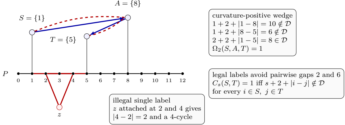
Figure 17: Visual definition of the P_{13} label algebra and the two-step curvature tensor. The black horizontal path is the induced P_{13} , with indices 0, \dots, 12 displayed below its vertices. An outside vertex has label equal to the set of path indices to which it is adjacent. The lower red vertex z illustrates an illegal label: attachments at indices 2 and 4 close a 4-cycle through the subpath v_2v_3v_4 , so legal labels must avoid pairwise gaps 2 and 6. The upper vertices carry the singleton labels S = \{1\} , A = \{8\} , and T = \{5\} . The blue outside edges show the two individually safe length-1 relations C_1(S, A) = 1 and C_1(A, T) = 1 . The dashed red two-step outside path from S to T , together with the red path segment v_1 \cdots v_5 and the two attachment edges, has length 2 + 2 + |1 - 5| = 8 ; hence C_2(S, T) = 0 . Thus \Omega_2(S, A, T) = 1 : two locally safe outside steps compose into an unsafe dyadic test.
