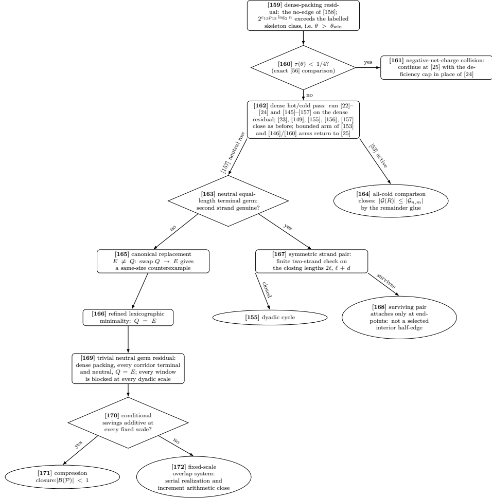
Figure 12: Proof-dependency diagram, Part XII. The dense residual [159] passes through the exact deficiency test [160] and the dense hot/cold pass [162]. The all-cold arm closes at [164]; the neutral arm [163] splits into the replacement route [165]–[166] and the two-strand route [167], [155], [168]. The continuation of [166] is included here: the trivial neutral residual [169] reaches either compression [171] through additivity [170], or the serial-system arithmetic closure [172].
