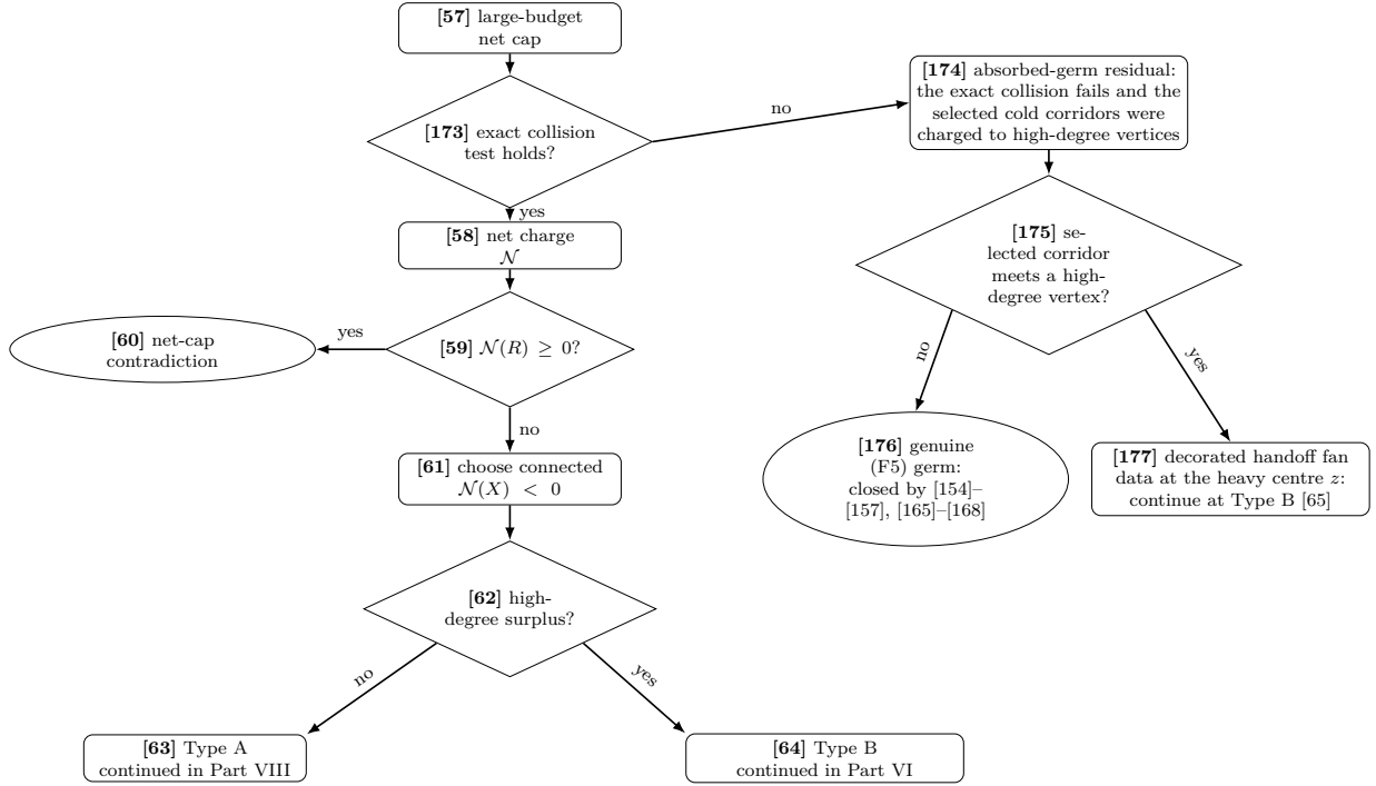
Figure 5: Proof-dependency diagram, Part V. Conventions are as in Fig. 1. This panel performs the net-charge split [57]–[64] and expands the no-edge of [173] in place. Node [173] is the exact net-cap collision test of Lemma 7.28; its failure gives the absorbed-germ residual [174]. Node [175] restores the discarded charge by Lemma 7.29: a selected corridor with no high-degree vertex is a genuine (F5) germ and closes at [176], while the other branch supplies decorated handoff fan data and enters Type B [65] at [177]. Node [63] continues in Fig. 8, and nodes [64] and [177] continue in Fig. 6.
