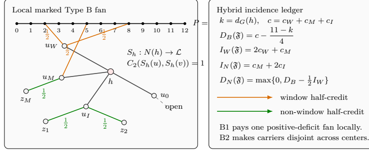
Figure 27: Visual definition of the Type B fan-window and hybrid ledger data. The left panel is the local marked Type B fan, with high-degree center h and neighbours in N(h) ; the right panel is the hybrid incidence ledger. The horizontal black path P = p_0 \cdots p_{12} is a packed induced P_{13} window, with the displayed indices naming its vertices. The labelling S_h : N(h) \rightarrow \mathcal{L} assigns fan certificates, and the condition C_2(S_h(u), S_h(v)) = 1 states pairwise fan-safety for distinct neighbours. The neighbour u_W is window-supported because both of its non- h incidences go to window vertices; u_M is mixed-supported because one incidence goes to the window and one to a non-window vertex z_M ; u_I is internal-supported because its two non- h incidences go to non-window vertices z_1, z_2 ; and u_0 is an open neighbour, so it is not counted as cubic-closed in this local ledger. Orange edges are window incidences, green edges are non-window incidences, and each displayed \frac{1}{2} is the half-credit contributed by one such incidence. In the ledger, k = d_G(h) , c = c_W + c_M + c_I counts cubic-closed neighbours by support type, D_B(\mathfrak{F}) = c - (11 - k)/4 is the closed-neighbour deficit, I_W = 2c_W + c_M is the window-incidence count, I_N = c_M + 2c_I is the non-window-incidence count, and D_N = \max\{0, D_B - \frac{1}{2}I_W\} is the remaining non-window demand. B1 denotes the local payment of one positive-deficit fan, while B2 denotes the cross-center disjointness ledger needed to sum those payments globally. The bottom boxed note records the alternate case: if the labelling S_h is absent, then h is charged as a fan-certificate residual center in the Type B fan-mass ledger.
