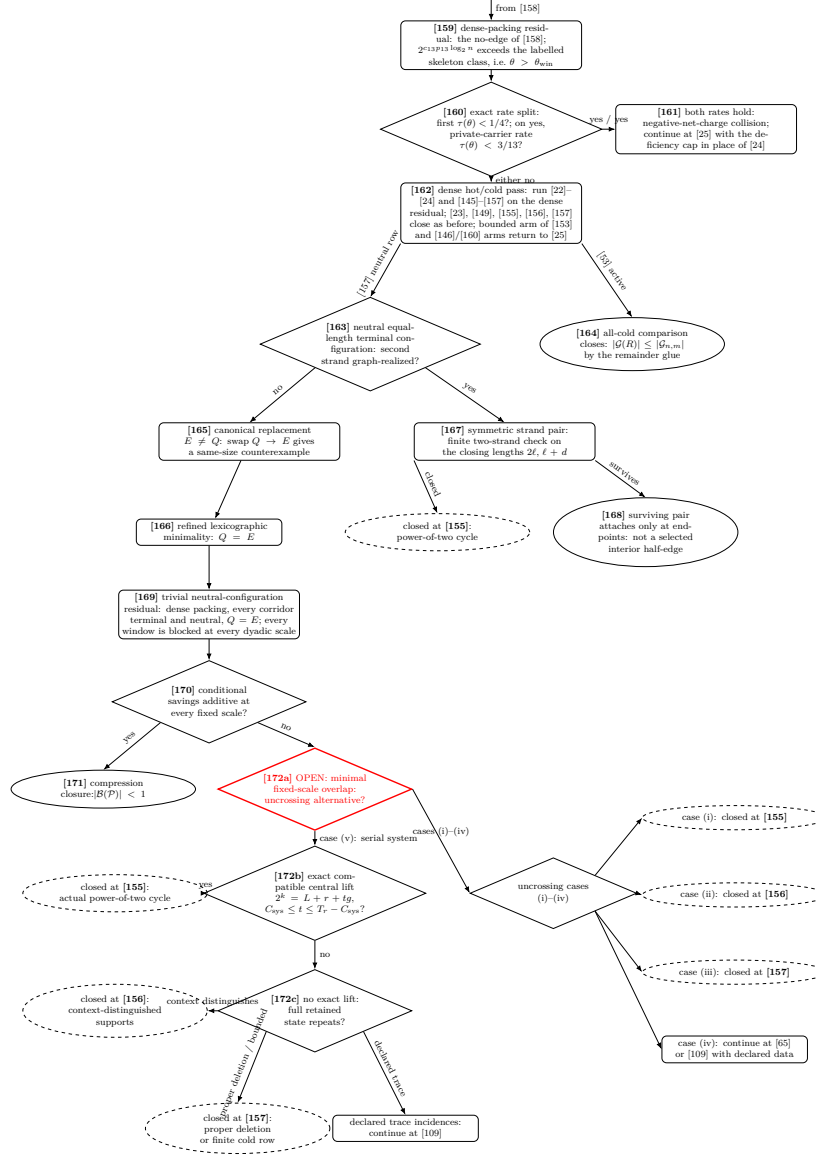
Figure 12: Proof-dependency diagram, Part XII. The dense residual [159] passes through the two exact rate tests at [160]. Only the arm satisfying both the net-deficiency rate \tau(\theta) < 1/4 and the route-8 private-carrier rate \tau(\theta) < 3/13 enters [161]. Failure of either comparison enters the dense hot/cold pass [162] on its literal residual. The all-cold arm closes at [164]; the neutral arm [163] splits into the replacement route [165]–[166] and the two-strand route [167], [155], [168]. The dashed ellipses are closure proxies for the solid terminals [155]–[157] in Fig. 11, not additional proof nodes. The continuation of [166] is included here: the trivial neutral residual [169] reaches compression [171] through the yes-arm of [170]. Its no-arm retains the failing fibre and minimal connected overlap support and enters the typed node-[172] subdiamond. Node [172a] uncrosses the overlap; alternatives (i)–(iv) carry their actual G1/G2/G3 or declared-handoff witnesses to the existing destinations, while alternative (v) supplies the serial system and its residue-specific ranges to [172b]. The yes-arm of [172b] is an exact compatible central lift and hence an actual power-of-two cycle [155]. Its literal complement enters [172c] with the full residue modulo g , cold cut state, boundary-degree profile, truncated end distances, fixed rare choices, and declared trace incidences. A context-distinguished repeat closes at [156], an exhibited target-complete proper deletion or a genuinely bounded no-repeat row closes at [157], and a repeated declared trace support continues with its indexed carrier data at [109].
