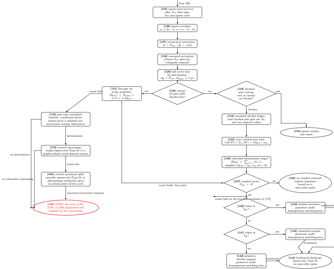
Figure 10: Proof-dependency diagram, Part X. This panel expands the sparse non-near-cubic branch [20]. Nodes [126]–[129] build the full active surplus family. Node [130] splits canonical pairs. Free pairs are charged by the entropy sandwich [131], while blocked pairs pass through the blocker route [132]–[136]; the role fibres in [136] partition \Pi_{\text{blk}} , so this ledger has no double counting. Node [137] is the coupled single-graph test of Corollaries 3.53 and 3.54 and Proposition 3.55 : all three token classes use the same n, p_{13}, \sigma_W, \sigma_R . If D_{\text{all}} = 0 , the explicit quadratic bound routes to [138]. If D_{\text{all}} > 0 , the role-fibre excess enters the window-incidence, remainder-surplus, or primitive blocker-support geometric audit [140], [142], [143]. Node [144] applies Theorem 3.78 : the bottleneck realizes a sparse surplus exit, produces Type B fan data, or is bounded by fixed homogeneous caps and routes to [138]. The entropy counts of [131] and of the free side of [137] are branch tests. On the covered pair-code arm, [178] retains the exact conditional factorization and minimal connected overlap obstruction, [179] retains either an already routed outcome or the graph-realized serial system, and [180] retains either an already routed periodic outcome or the exact full-modulus arithmetic data from which an actual power-of-two cycle is constructed. The manuscript does not prove that these three classifications are exhaustive on the retained residual. Their literal failures therefore meet only at the explicit open node [182]; none is renamed as a blocker, quotient, exit, or Type B witness.
