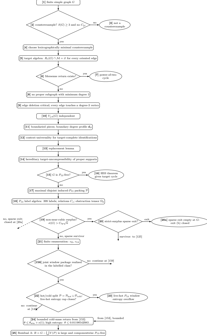
Figure 1: Proof-dependency diagram, Part I. Rectangles are assertions or residual states, diamonds are exhaustive branch tests, ellipses are terminal outcomes, and edge labels state which branch is followed. The bracketed numbers are unique diagram-node numbers used by the dependency table. Nodes [19] and [20] record the non-near-cubic surplus accounting branch used before the normalized spine budget; the strict surplus sparse exit reaches [20a], which is closed because exit (b) is empty at G (Lemma 3.27), so only the strict-surplus survivor continues at [125] in Fig. 10. On the at-or-below arm, the sparse exit closes at [20a] in the same way, while the sparse survivor enters [21]. Node [158] is the exact finite form of the realization sentence of Lemma 7.1 and Proposition 7.42: it asks whether the joint window package of the fixed maximal packing is realized by the labelled skeleton class; its no-branch is the dense-packing residual expanded in Fig. 12. Node [22] creates the hot/cold dichotomy by splitting \mathcal{P} into \mathcal{P}_{\text{hot}} and \mathcal{P}_{\text{cold}} . Its no-branch continues at [145] in Fig. 11. The bounded arm of [153] returns to [24] with the density cap, and only that live residual continues to [25] and Fig. 2.
