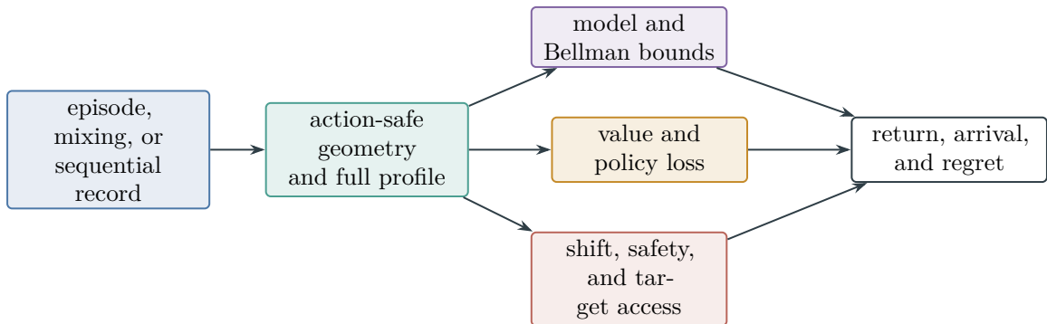
Figure 98: The learned-control certificate propagates one completely charged trajectory record through action-safe geometry. Generalization, functional inequalities, policy loss, safety, and target access remain typed until a theorem converts them to return, arrival, or regret units.
