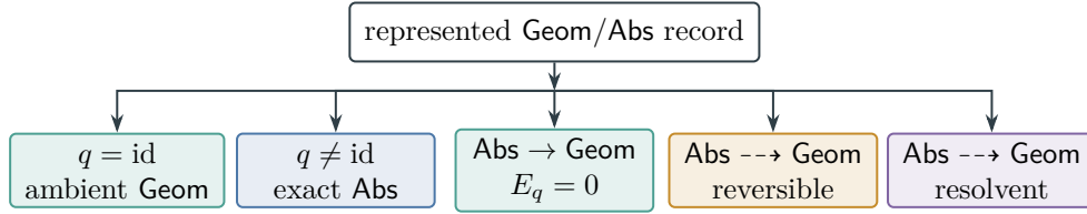
Figure 18: The compensated quotient-geometry certificate has five alternative configurations, classified by Theorem II.9.4.
