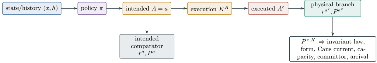
Figure 67: The physical controlled kernel is selected by the executed action. Averaging policy, execution channel, and physical transition produces P^{\pi,K} ; this actual kernel, not the intended comparator, determines the invariant law, Dirichlet form, current, capacity, committor, and arrival.
