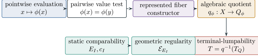
Figure 9: Observable interfaces have distinct types. Pointwise evaluation supplies value comparisons; a represented quotient additionally requires a charged fiber constructor. Terminal lumpability is a property of that quotient, whereas comparability and geometric regularity form an independent static interface.
