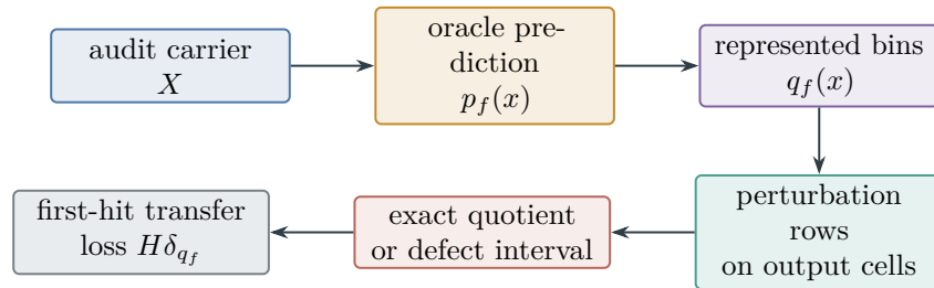
Figure 112: Behavioral quotient audit. Output cells become a dynamical abstraction only after their perturbation rows satisfy the exact or quasi-lumpability certificate.
