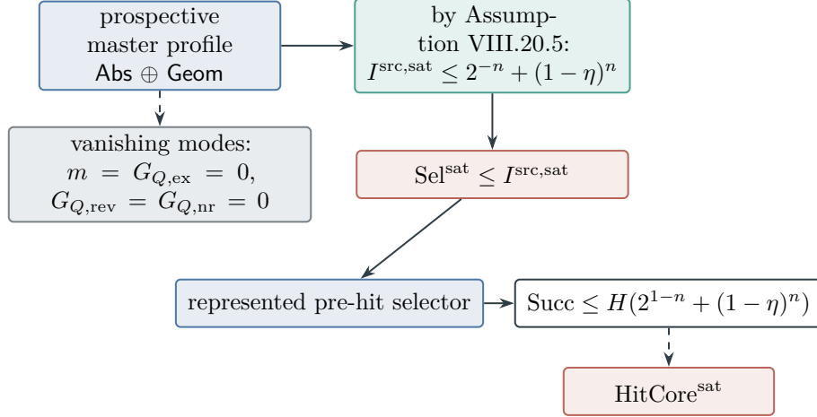
Figure 139: The exact LPN reduction. Exact abstraction and all three quotient-supported geometric modes vanish, and the complete saturated source profile is bounded at the common charged ceiling by Assumption VIII.20.5. Prospective selector accountability then gives the displayed success inequality. The separate HitCore coordinate retains completed first-hit accounting and is not a hardness hypothesis. The source and success bounds are Theorems VIII.21.1 and VIII.22.1.
