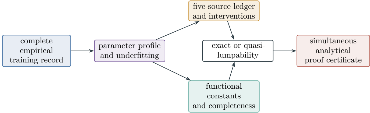
Figure 108: Empirical structural proof package. Parameter sufficiency, source-resolved learning, analytical functional inequalities, and quotient lumpability are certified from one completely charged record and one simultaneous confidence allocation.
