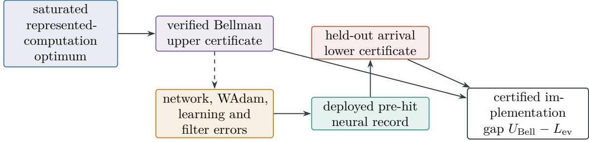
Figure 107: Certified neural realization of the saturated optimum. The deployed network supplies a primal lower certificate; a represented Bellman barrier supplies an upper certificate for the complete saturated class. Structural generalization, WAdam optimization, filtering, precision, and deployment are charged inside the common record.
