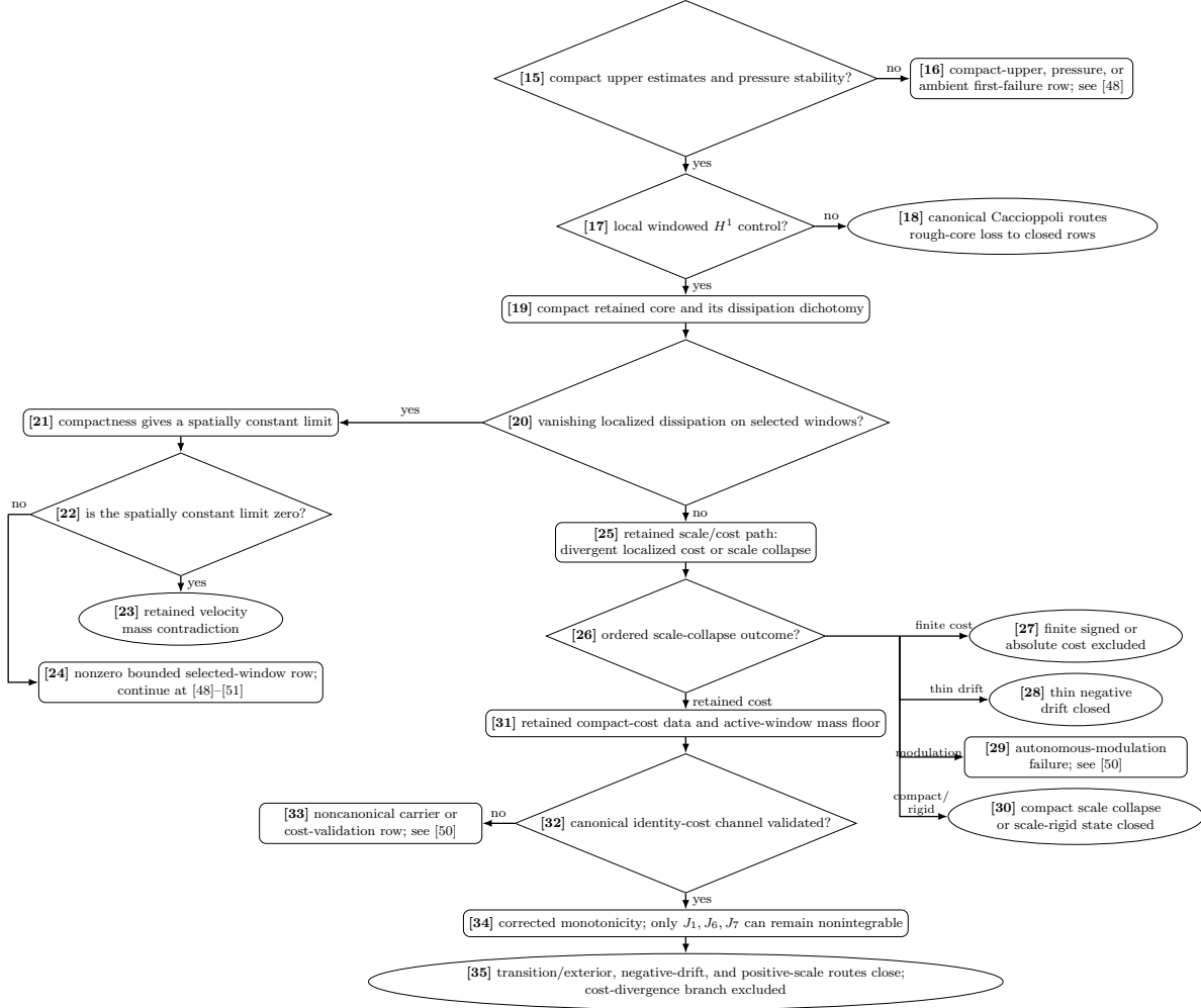
FIGURE 2. Type II proof-dependency diagram from compact-core tests through scale and localized-cost closure. Compact upper estimates and rough-core routing are supplied by proposition 7.14 and theorems 10.61 and 11.7 . At [20], the vanishing-dissipation branch is resolved by theorem 11.5 : [23] is a contradiction and [24] enters the bounded-window routing. The complementary branch enters [25] directly. The scale alternatives at [26] are those of theorem 11.9 ; nodes [27], [28], and [30] are closed by theorems 7.36 , 10.116 and 11.8 and proposition 5.42 . The canonical identity-cost channel is supplied by lemma 11.30 ; the remaining moving components are routed by theorem 8.133 before the cost-divergence exclusion is applied.
