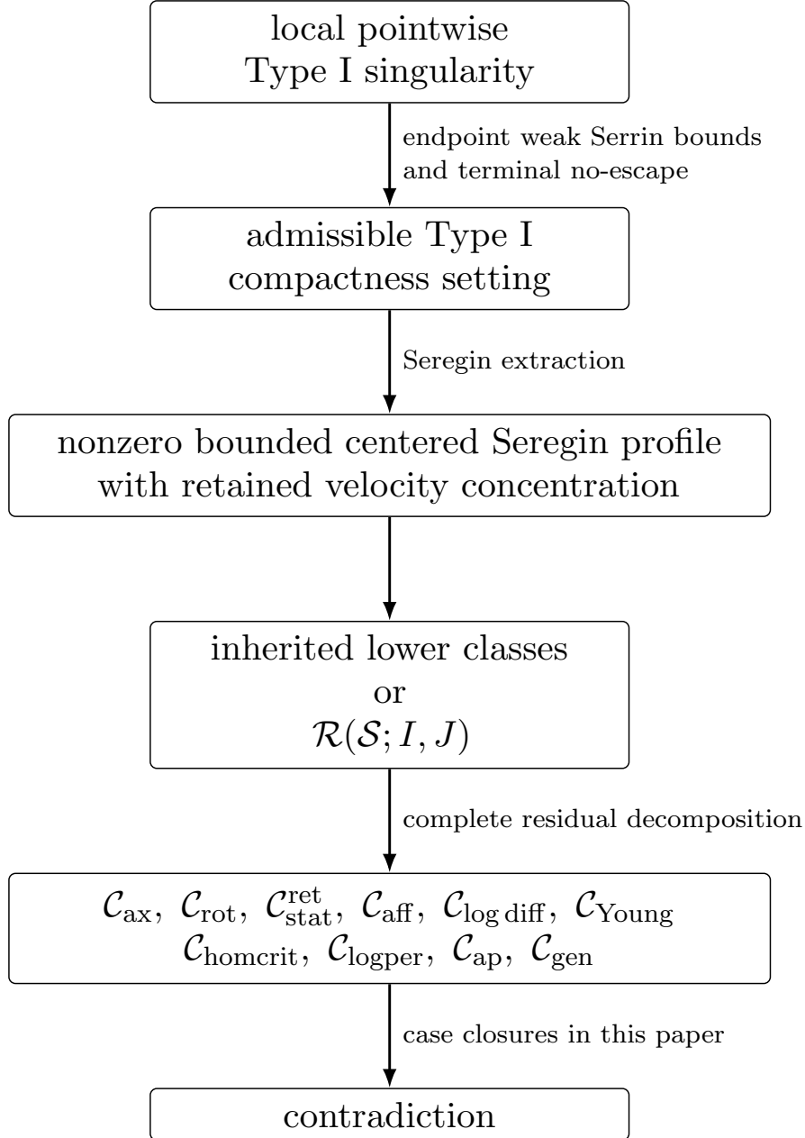
FIGURE 1. Compressed entry-to-closure view of the Type I profile decomposition. The first arrow uses the local pointwise Type I to terminal no-escape implication supplied by the endpoint weak Serrin estimate. The inherited lower classes are already closed in the setup paper. The boxed residual list is the refined classification of Definition 1.10 ; its routing and theorem-production orders are recorded separately in Tables 2 and 4 .
