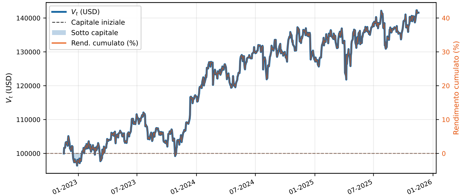
Punto 4.a — Buy-and-hold, cash 10%, 100,000 USD
