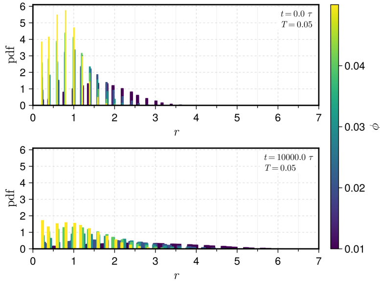
Figure 4: Comparisson of the distributions of the pore size for systems with different packing fractions at the initial configuration.
