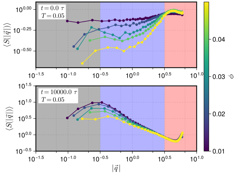
Figure 2: Comparisson of the structure factor for systems with different packing fractions. Grey area represent the large length scale, the blue area represent the intermediate length scale and the red area represent the small length scale. Top pannel is the initial configuration. The bottom panel is the final configuration after 10 \times 10^3 time units.
