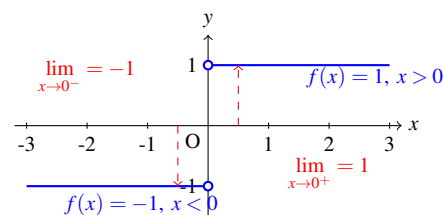
Figure 1: The circles indicates that the function is not defined at x = 0 .
