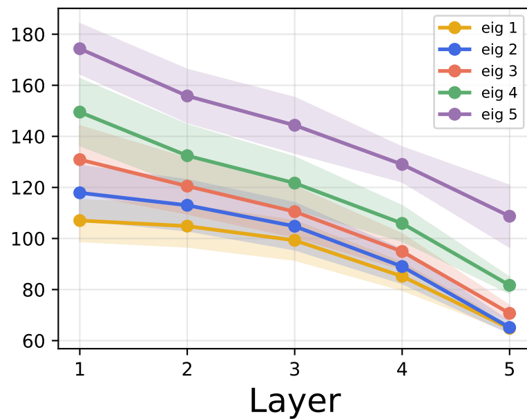
L2 norm
