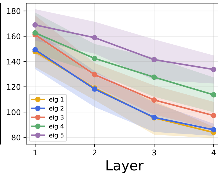
L2 norm
