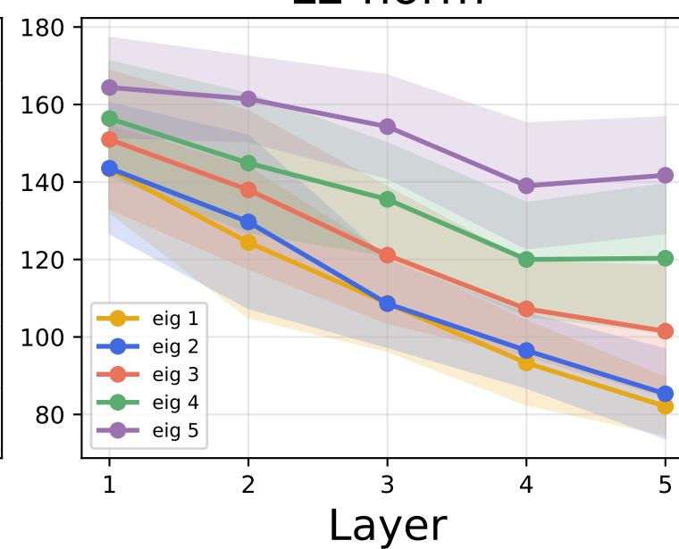
L2 norm
