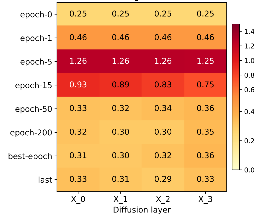
|Cohen's d| (accuracy, test set)
