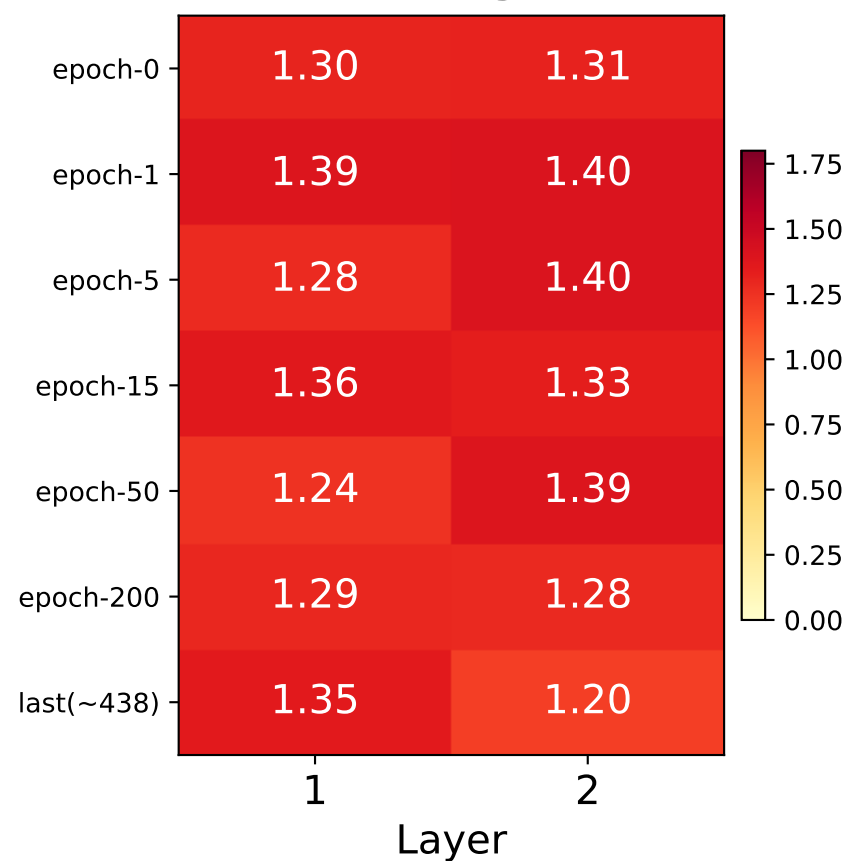
NRMSE
