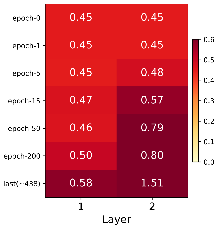
RMSE
