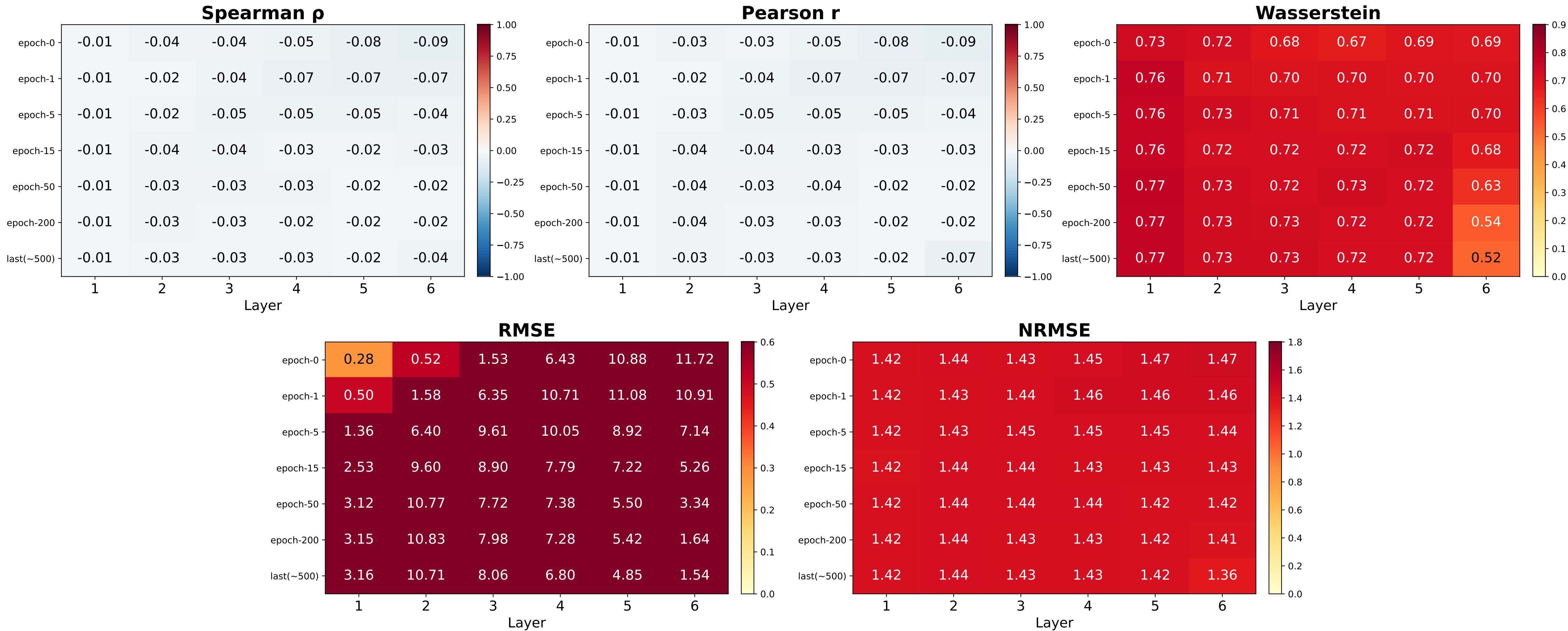
Forman Alignment Heatmap — minesweeper (GeneralSheaf, d=5, 6L, norm=False) (values = mean across 5 eigenvalues, averaged over folds)
