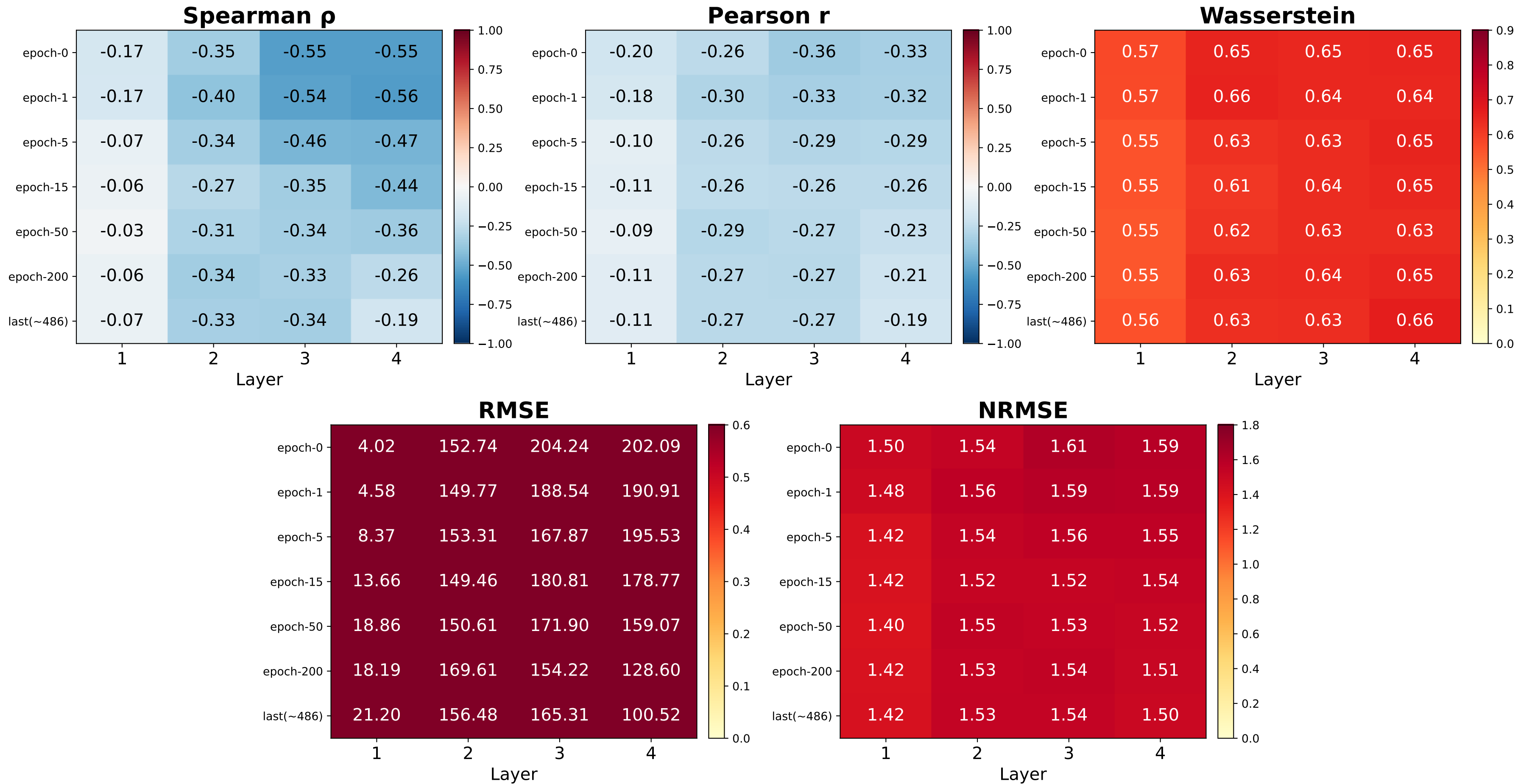
Forman Alignment Heatmap — tolokers (GeneralSheaf, d=3, 4L, norm=False) (values = mean across 3 eigenvalues, averaged over folds)
