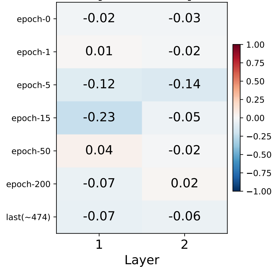
RMSE
