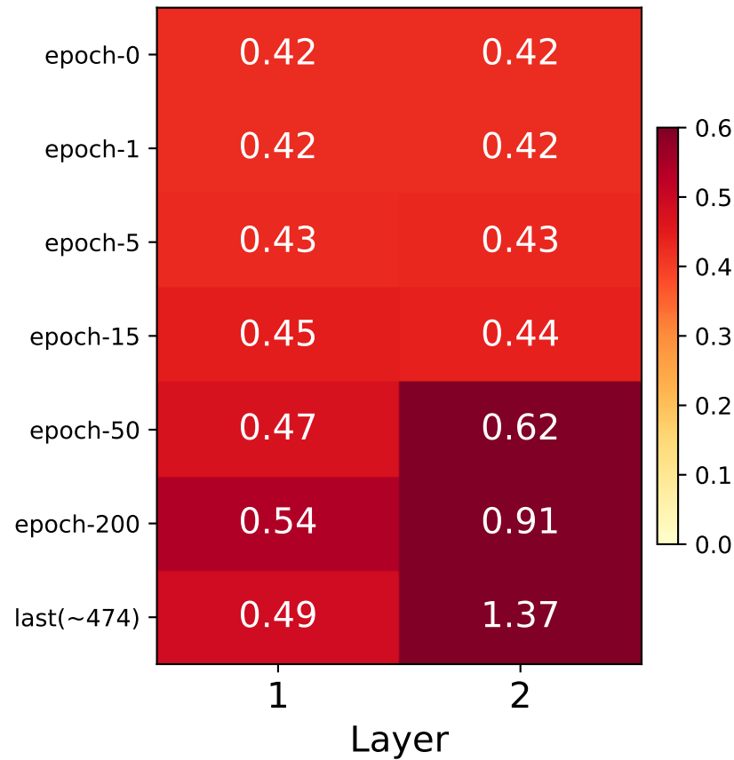
RMSE
