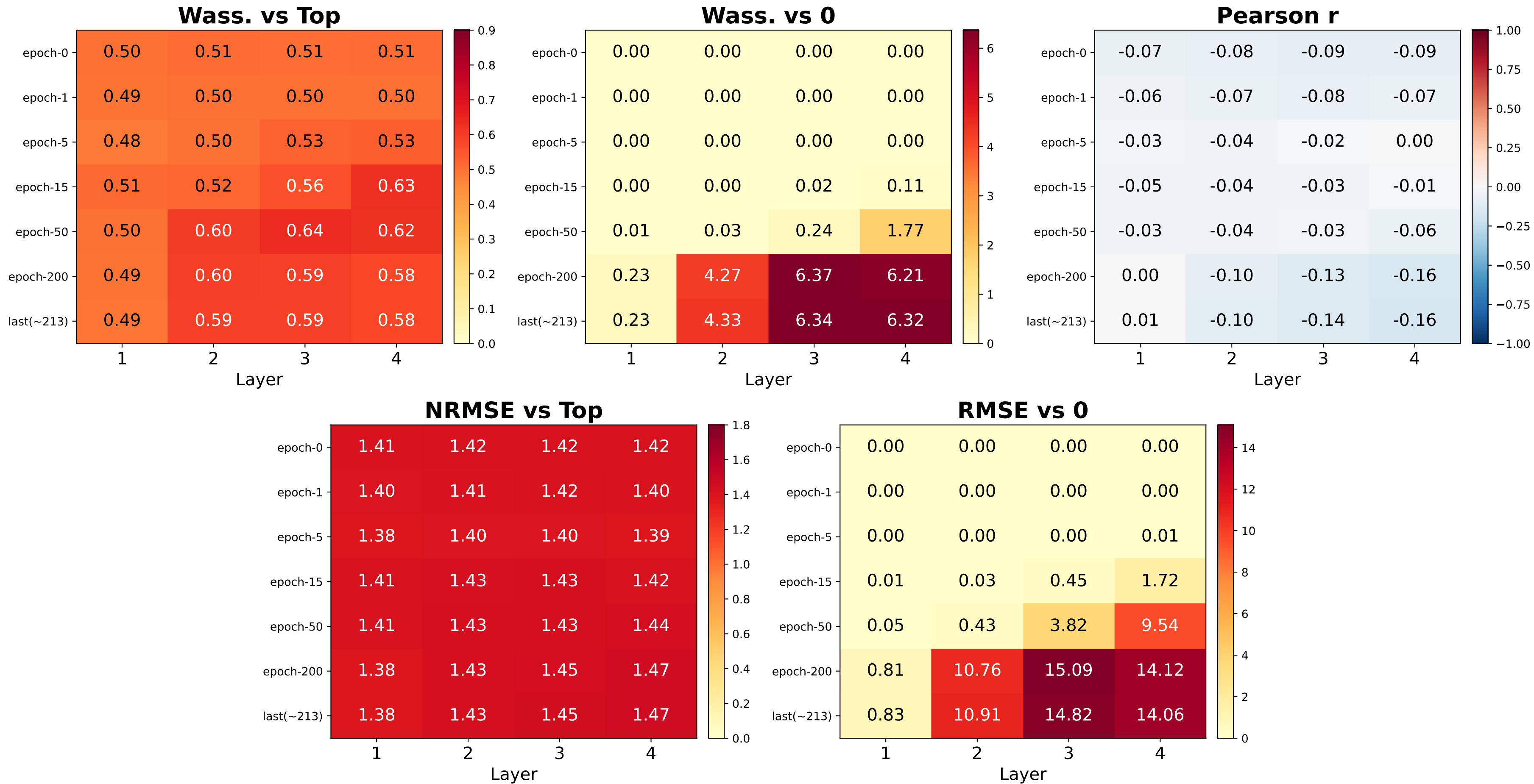
Forman Alignment Heatmap — pubmed (GeneralSheaf, d=5, 4L, norm=False) (values = mean across 5 eigenvalues, averaged over folds)
