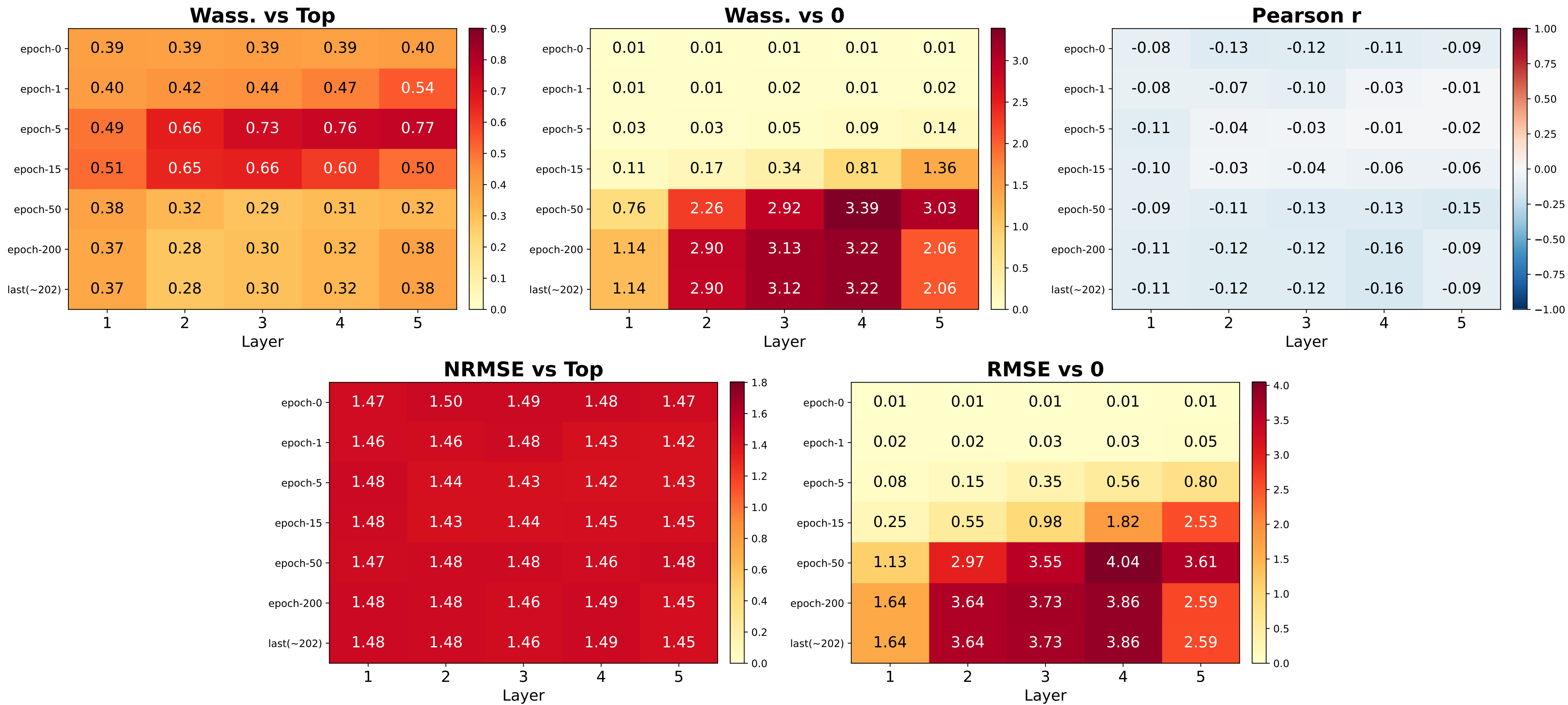
Forman Alignment Heatmap — roman_empire (GeneralSheaf, d=5, 5L, norm=False) (values = mean across 5 eigenvalues, averaged over folds)
