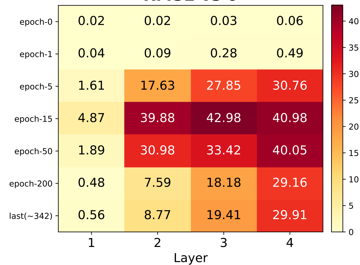
RMSE vs 0
