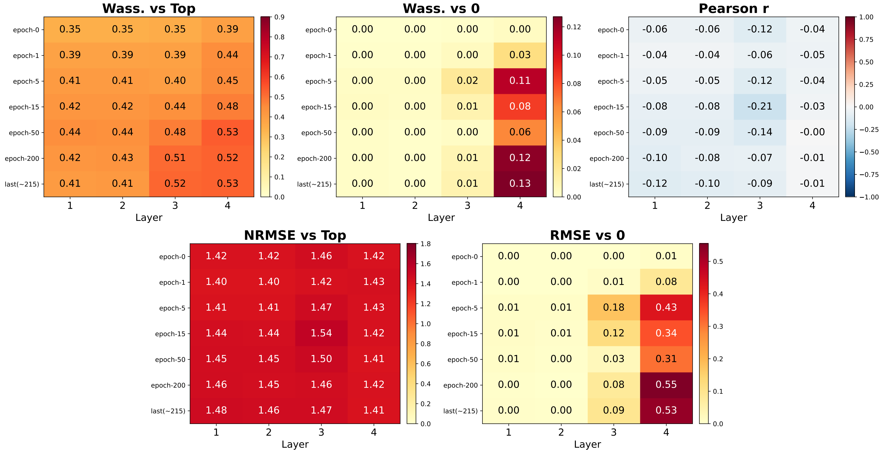
Forman Alignment Heatmap — citeseer (JointSheafParams, d=5, 4L, norm=False) (values = mean across 5 eigenvalues, averaged over folds)
