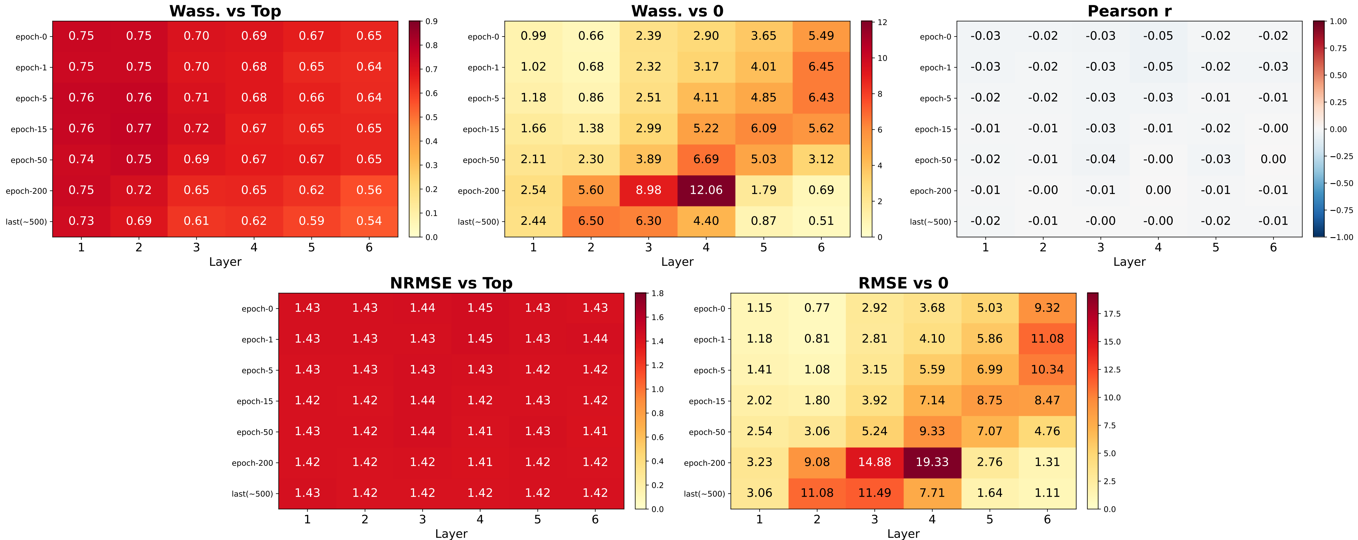
Forman Alignment Heatmap — minesweeper (JointSheafParams, d=5, 6L, norm=False) (values = mean across 5 eigenvalues, averaged over folds)
