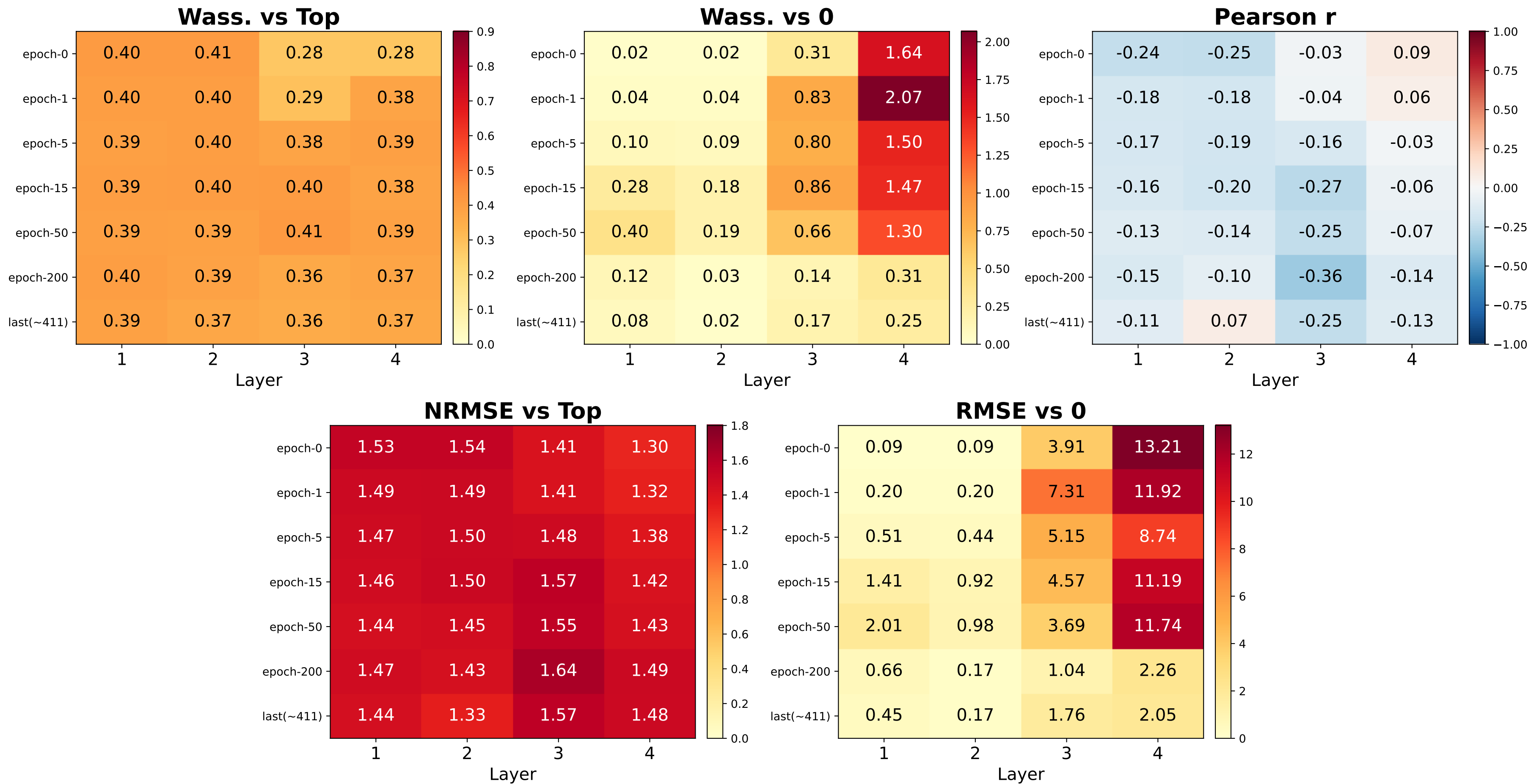
Forman Alignment Heatmap — questions (JointSheafParams, d=5, 4L, norm=False) (values = mean across 5 eigenvalues, averaged over folds)
