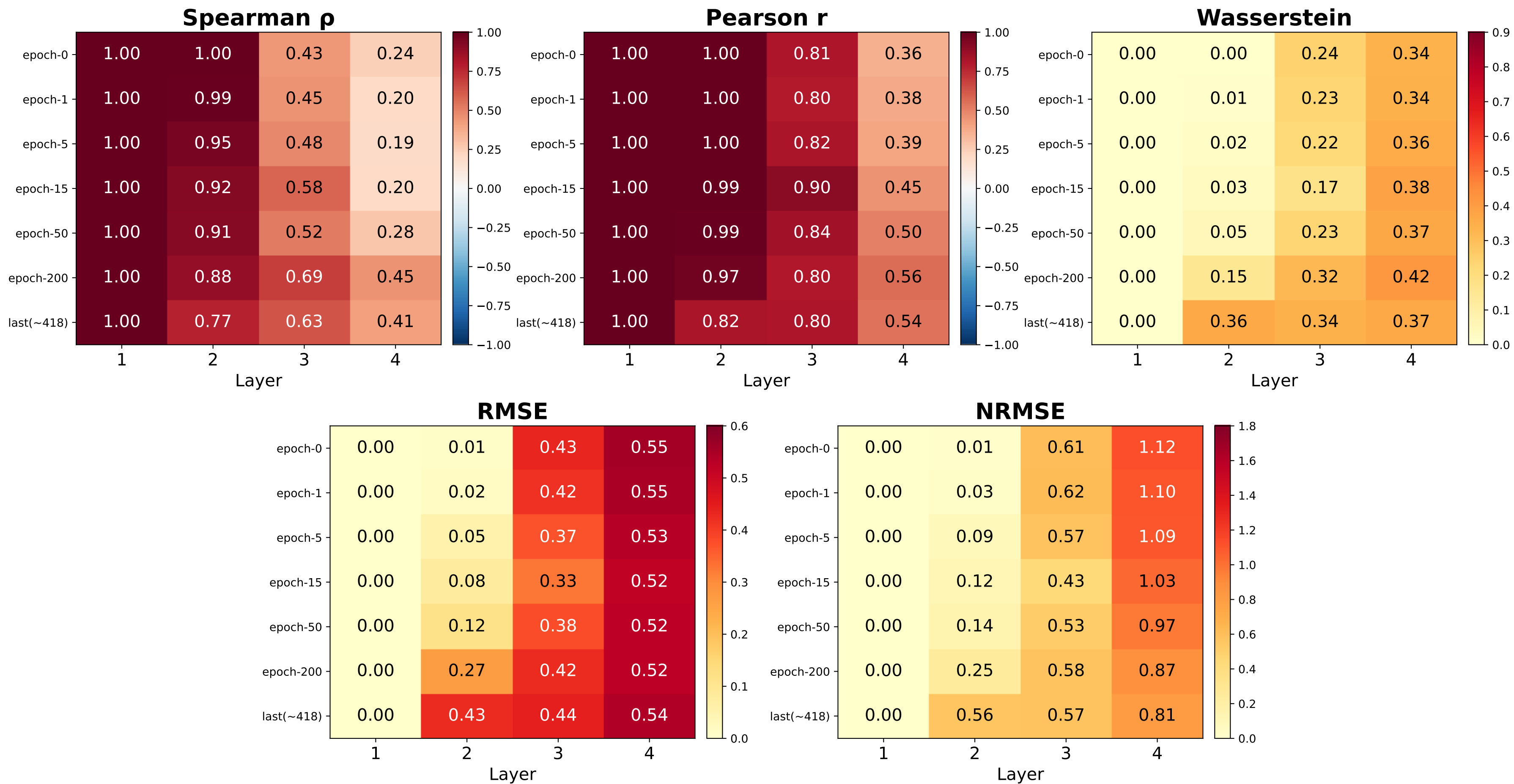
Forman Alignment Heatmap — questions (JointSheafParams, d=2, 4L, norm=True) (values = mean across 2 eigenvalues, averaged over folds)
