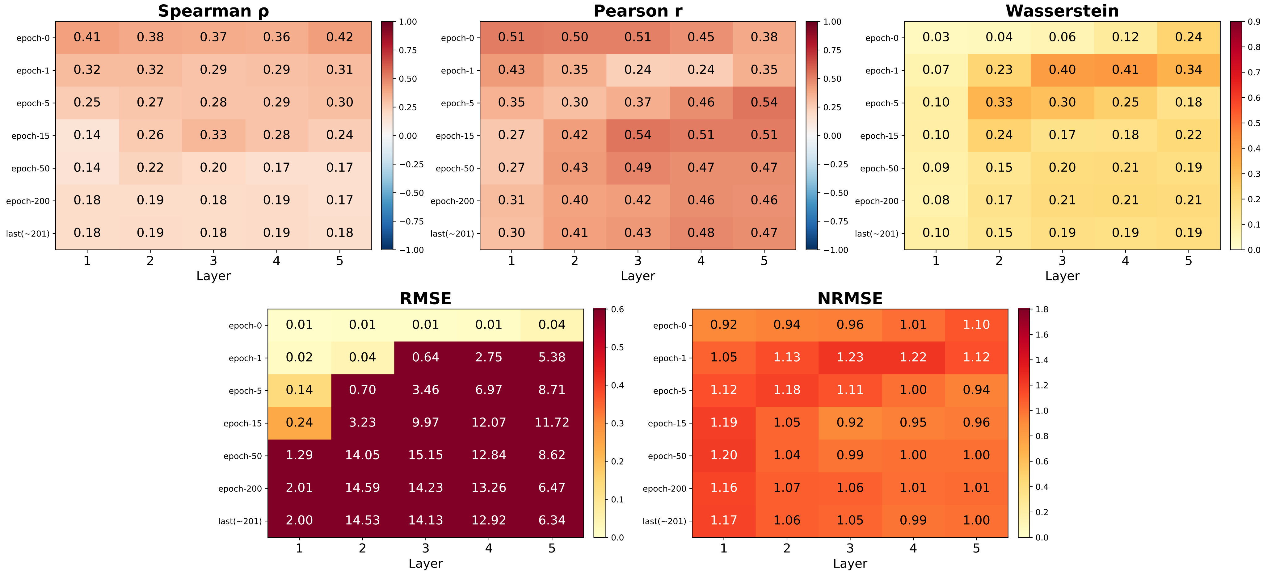
Forman Cross-Comparison — amazon_ratings (GeneralSheaf, d=5, 5L) norm_false_primary vs other_norm_true (values = mean across 5 eigenvalues, averaged over folds)
