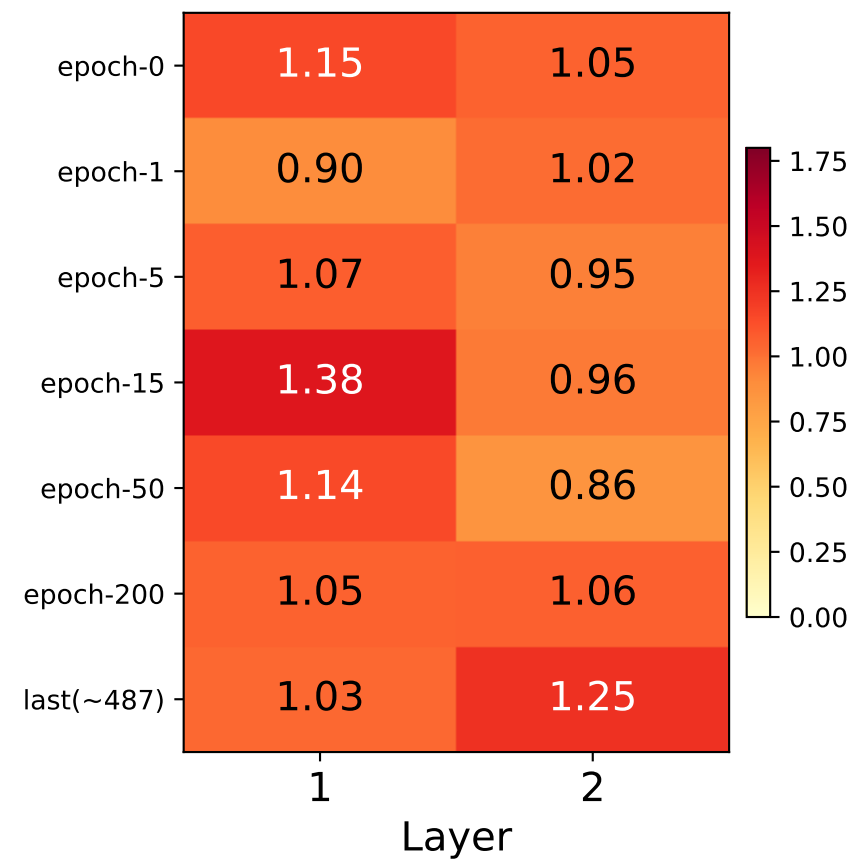
NRMSE
