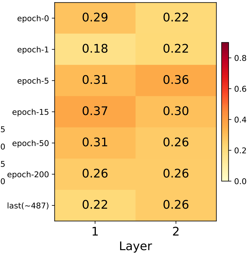
NRMSE
