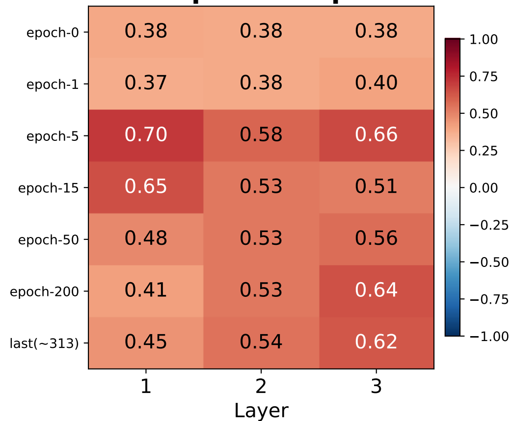
RMSE
