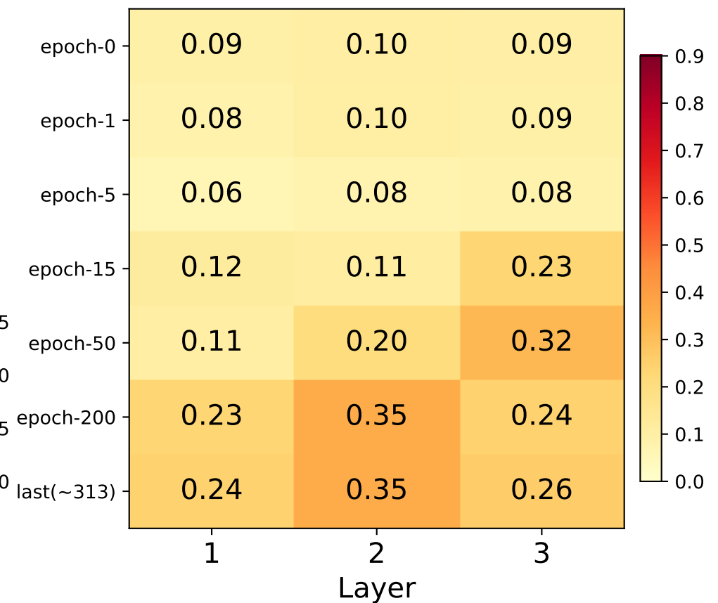
NRMSE
