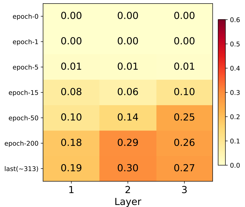
RMSE
