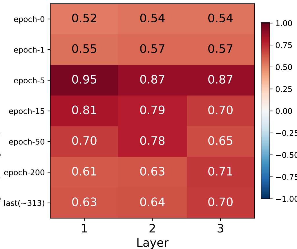
RMSE
