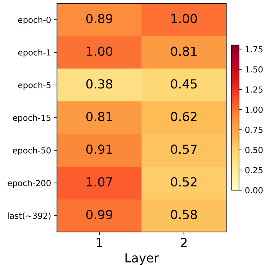
NRMSE
