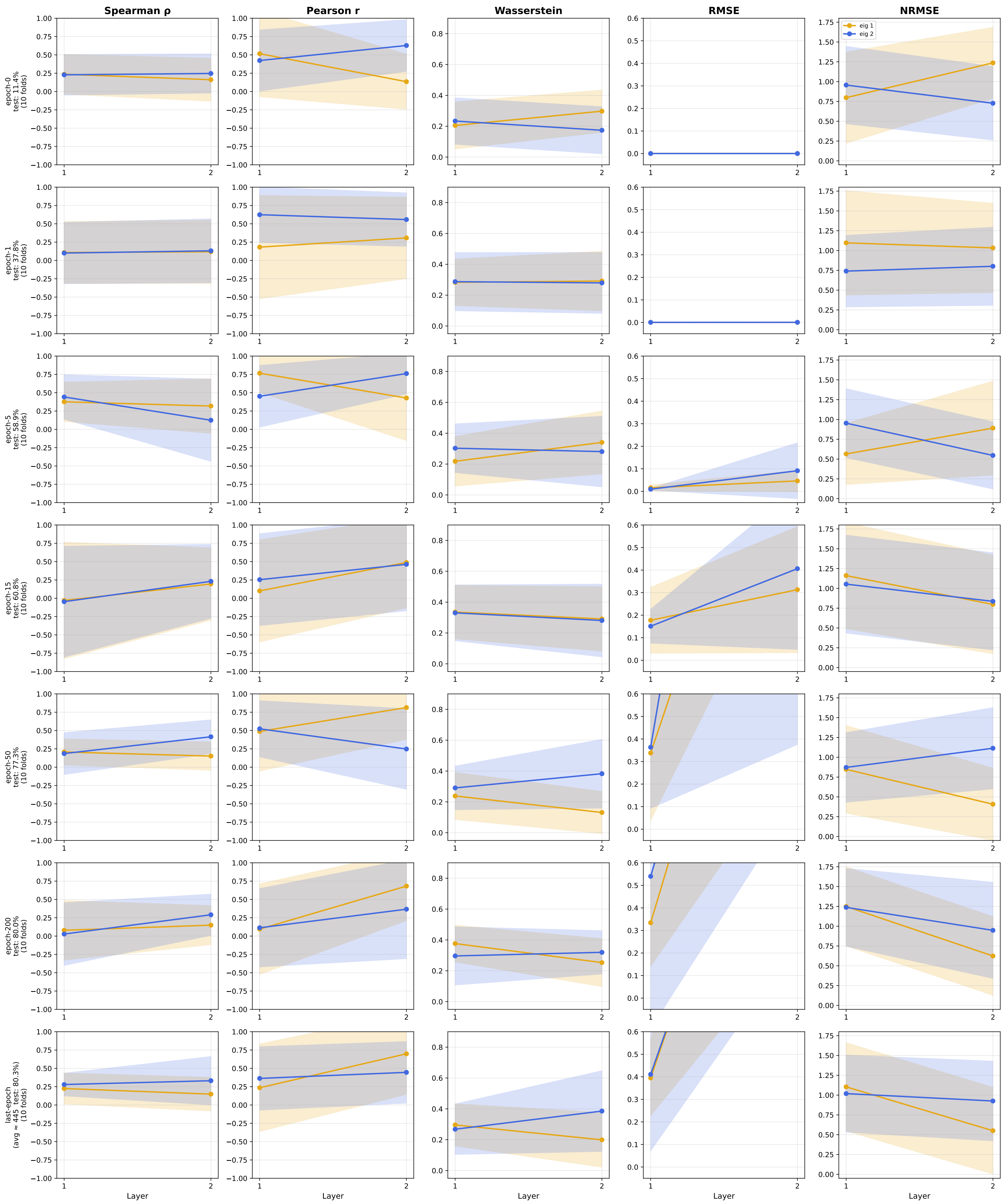
Forman Cross-Comparison — cornell (GeneralSheaf, d=2, 2L) norm_false_primary vs other_norm_true
