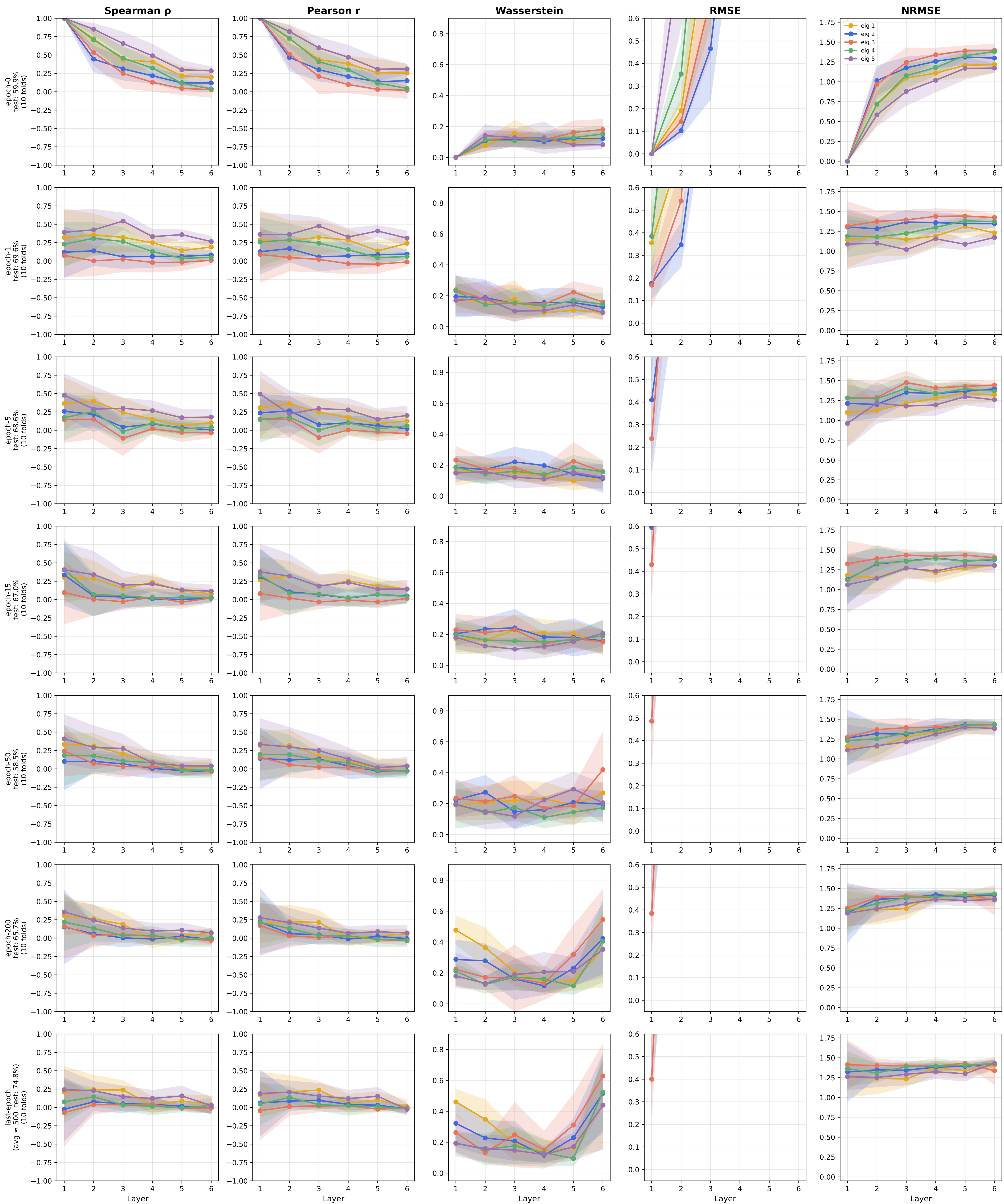
Forman Cross-Comparison — minesweeper (GeneralShear, d=5, 6L) norm_false_primary vs other_norm_true
