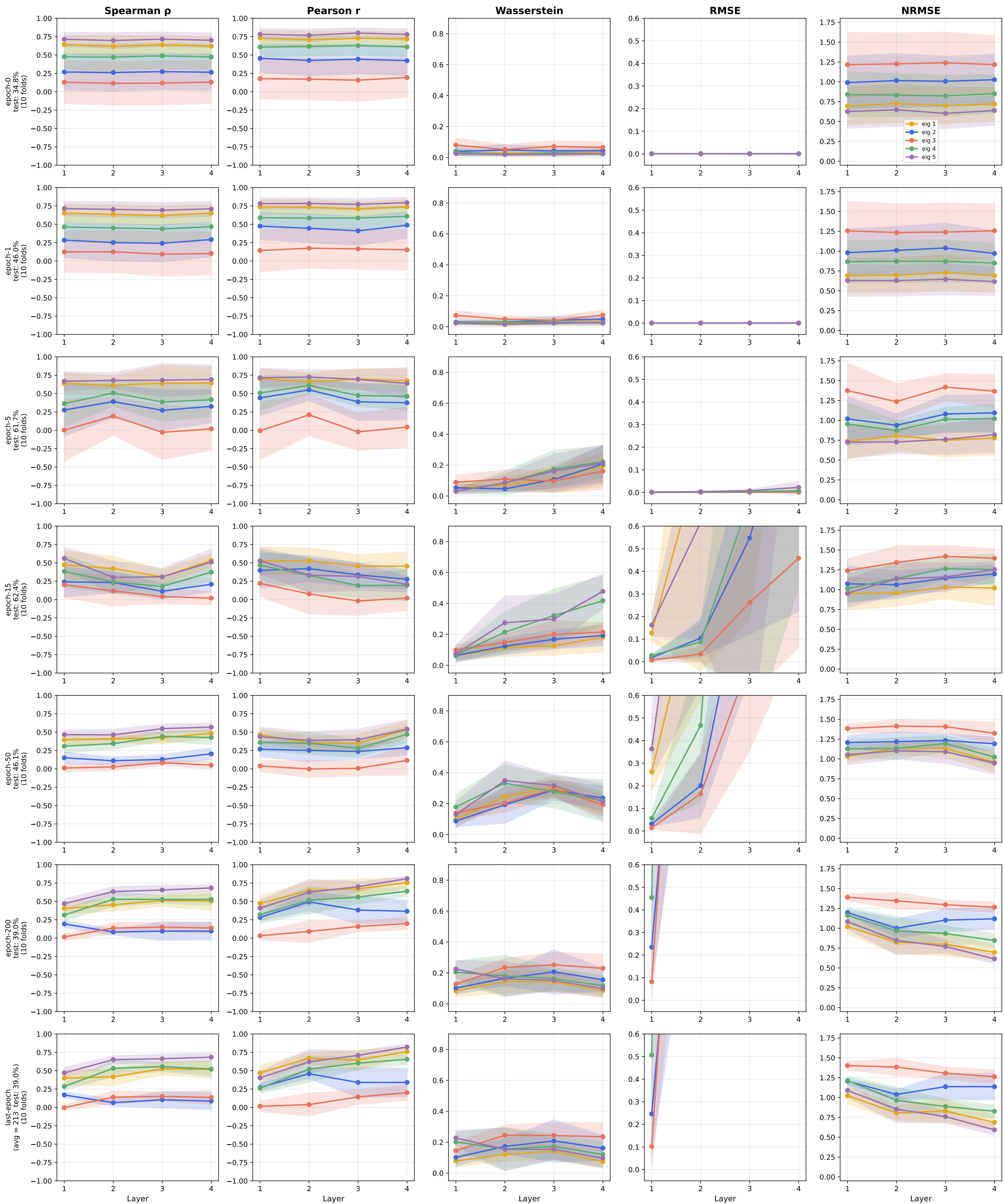
Forman Cross-Comparison — pubmed (GeneralSheaf, d=5, 4L) norm_false_primary vs other_norm_true
