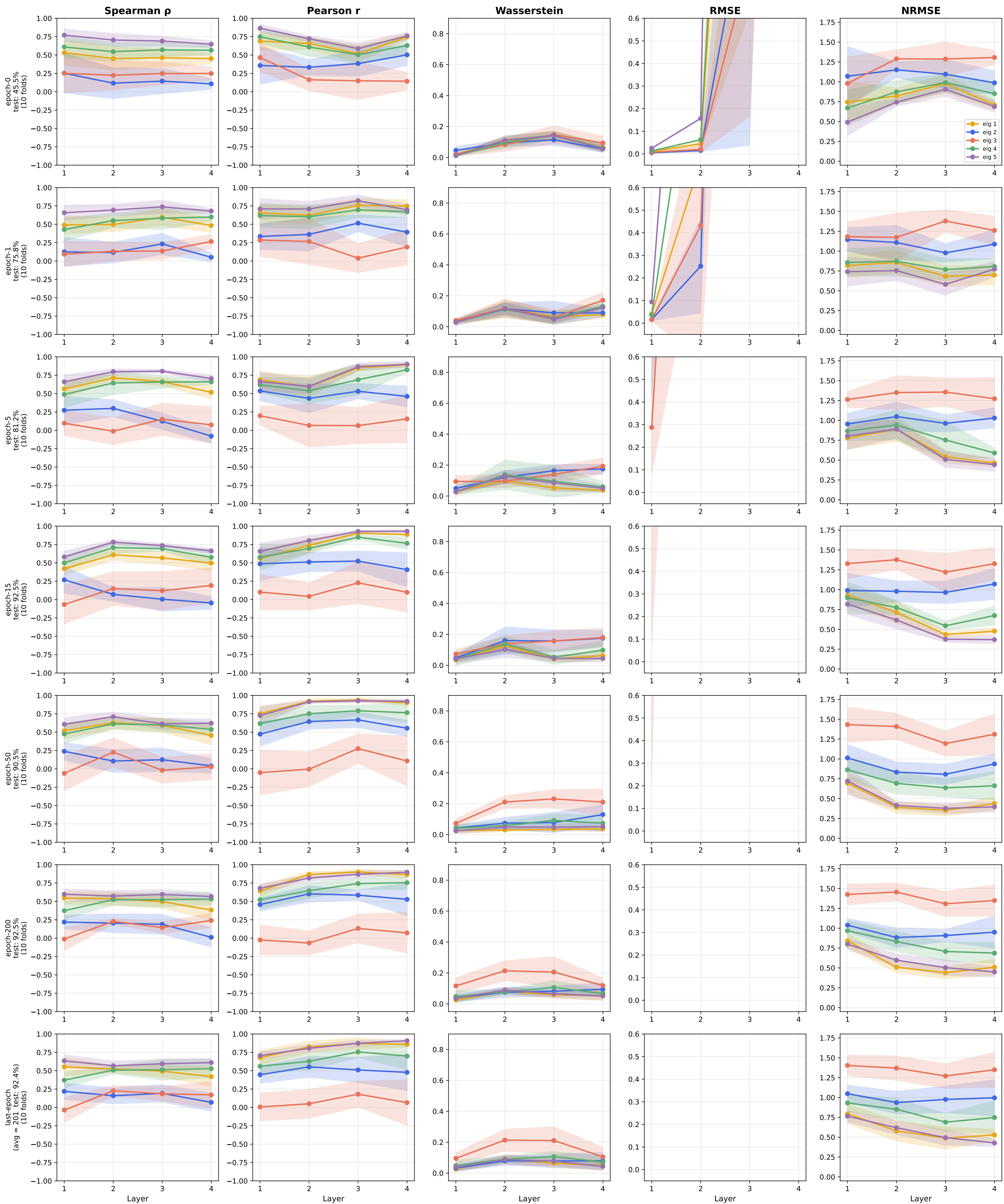
Forman Cross-Comparison — questions (GeneralSheaf, d=5, 4L) norm_false_primary vs other_norm_true
