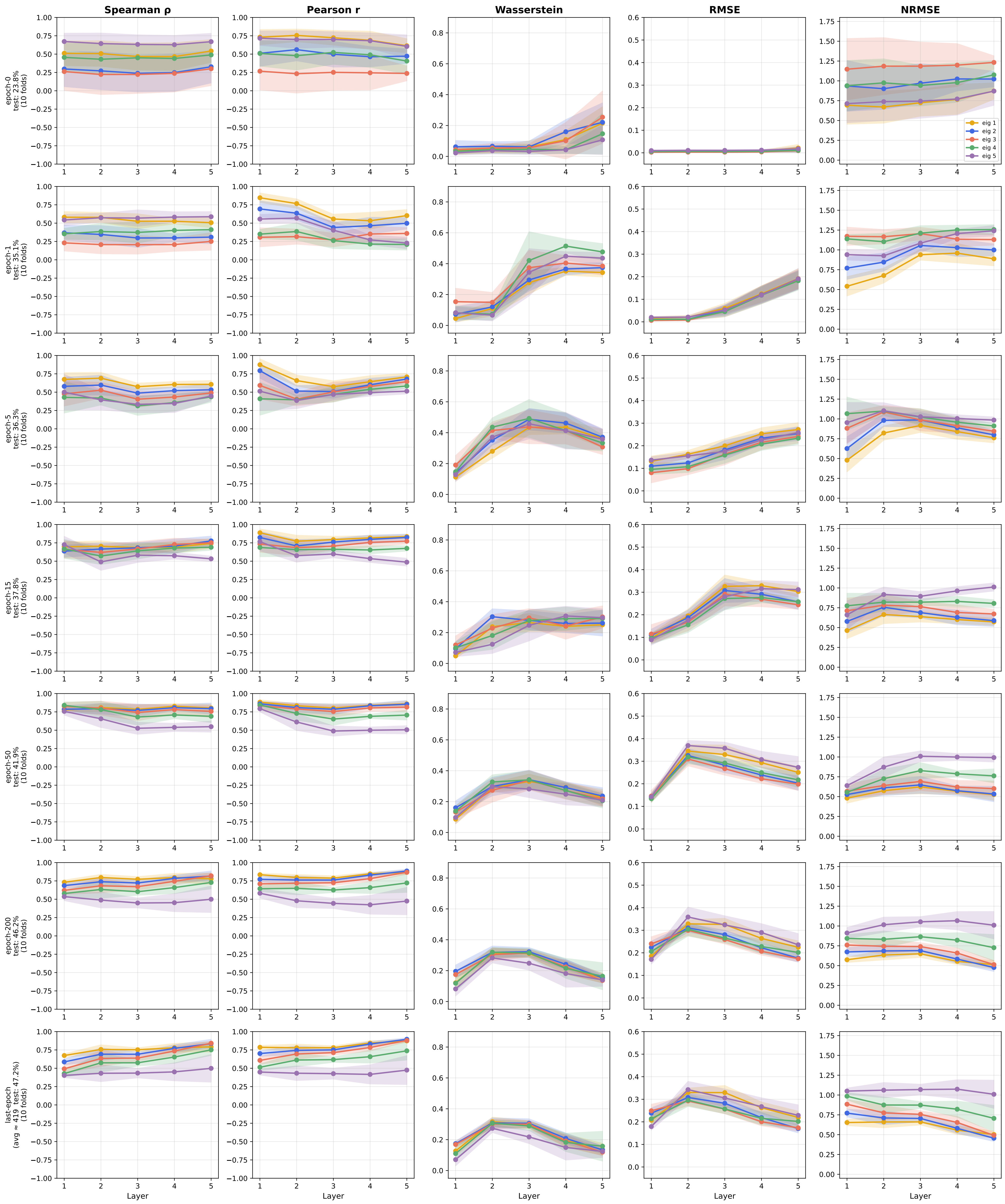
Forman Cross-Comparison — amazon_ratings (GeneralSheaf, d=5, 5L) norm_true_primary vs other_norm_false
