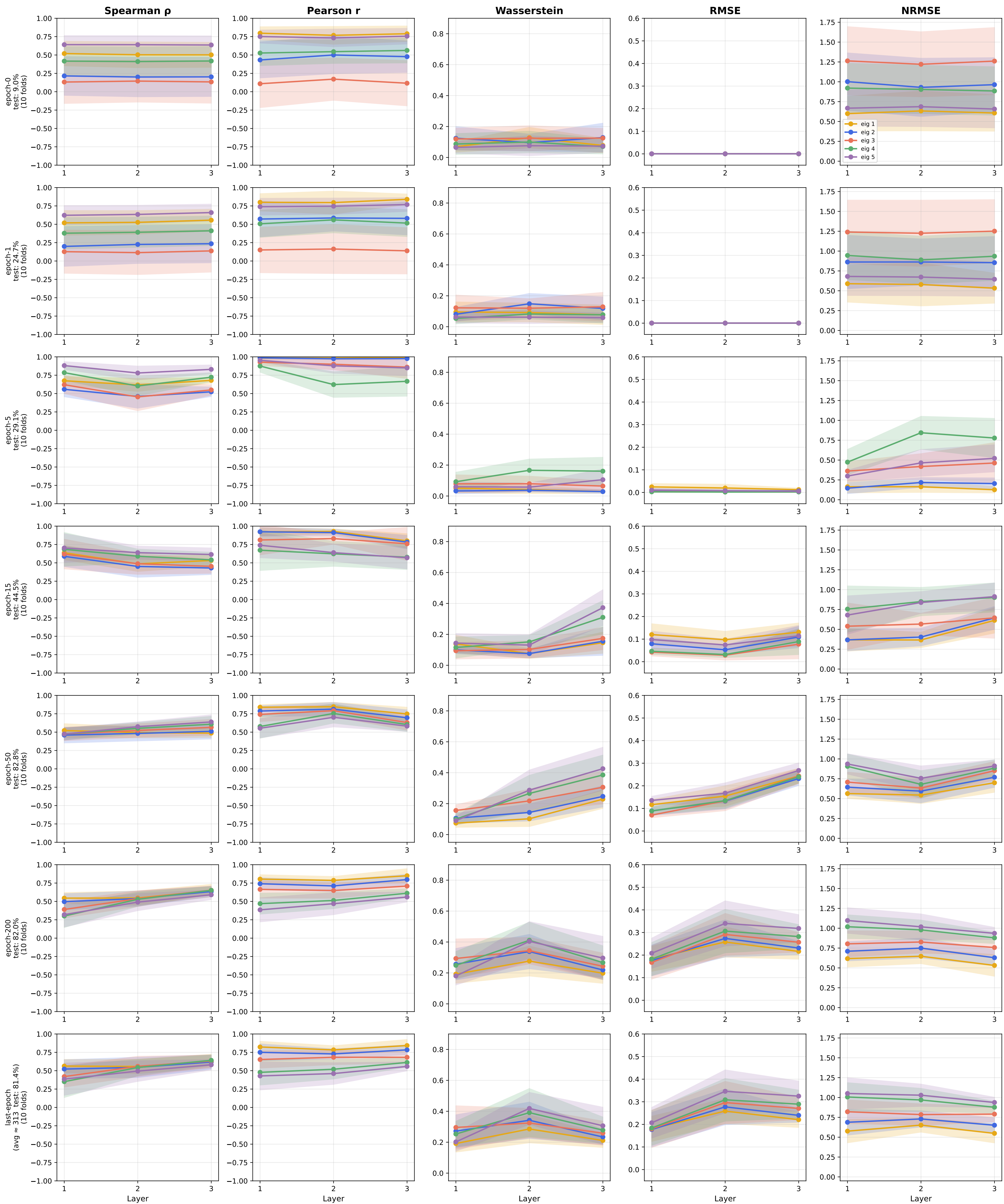
Forman Cross-Comparison — cora (GeneralSheaf, d=5, 3L) norm_true_primary vs other_norm_false
