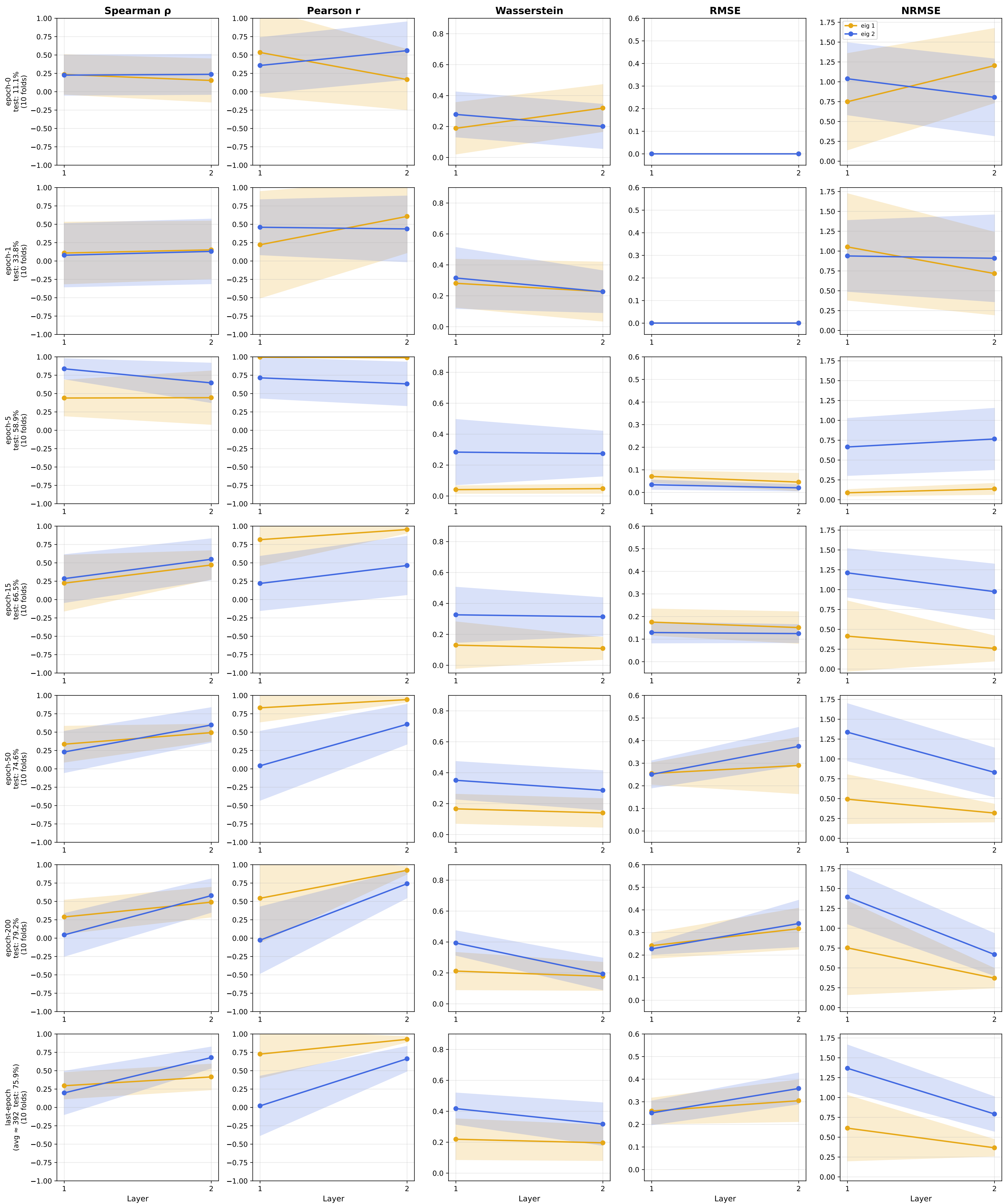
Forman Cross-Comparison — cornell (GeneralSheaf, d=2, 2L) norm_true_primary vs other_norm_false
