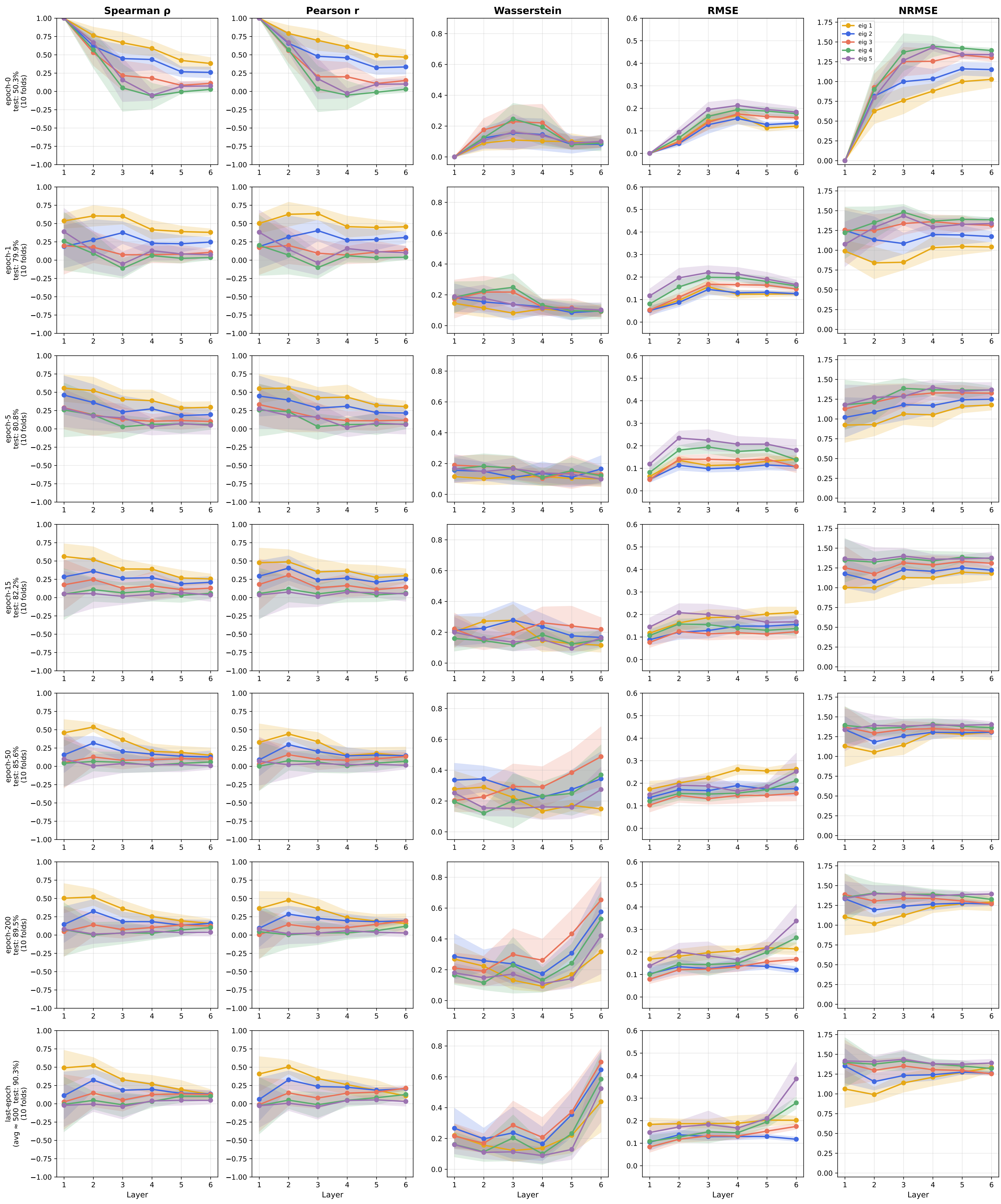
Forman Cross-Comparison — minesweeper (GeneralSheaf, d=5, 6L) norm_true_primary vs other_norm_false
