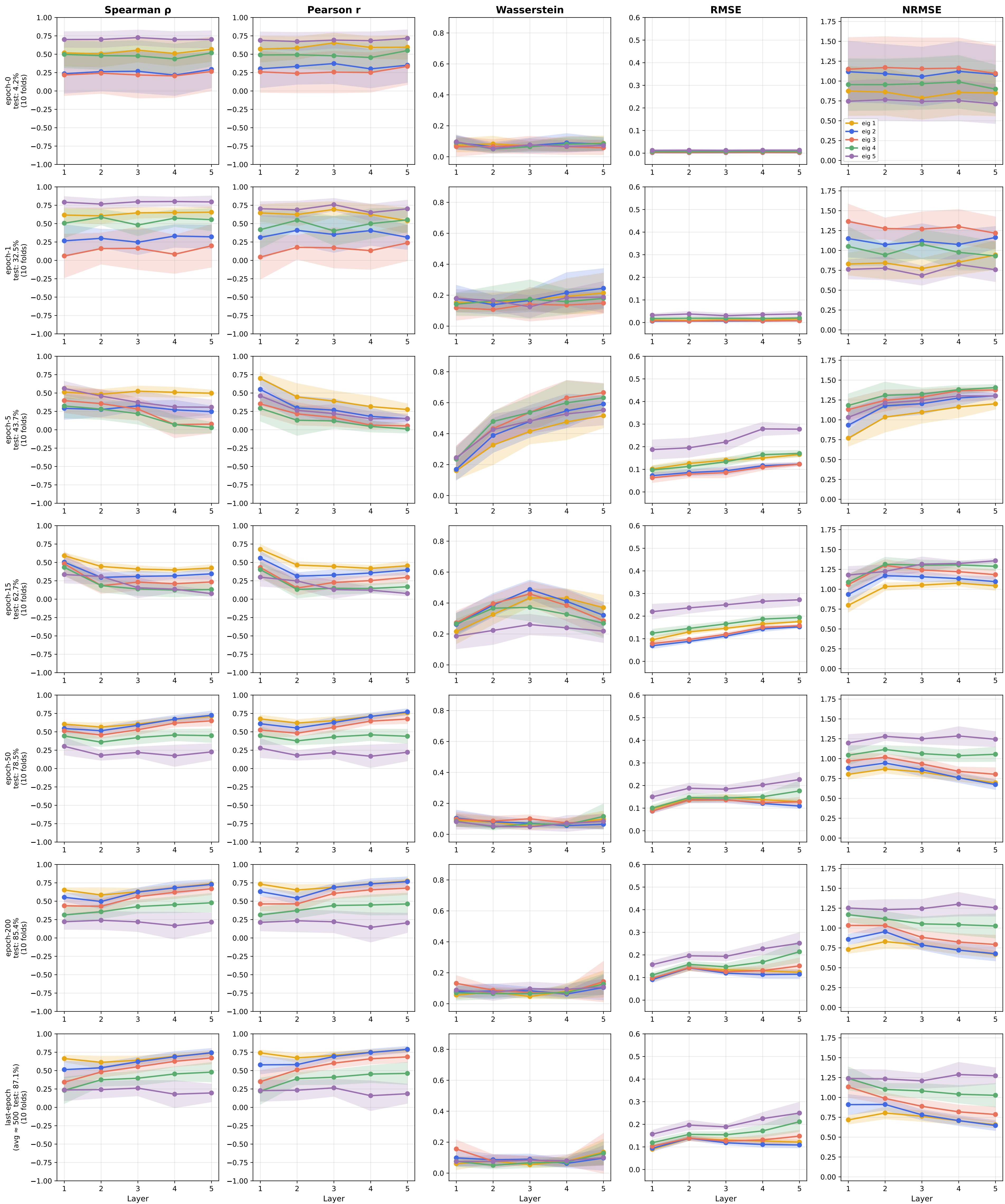
Forman Cross-Comparison — roman_empire (GeneralSheaf, d=5, 5L) norm_true_primary vs other_norm_false
