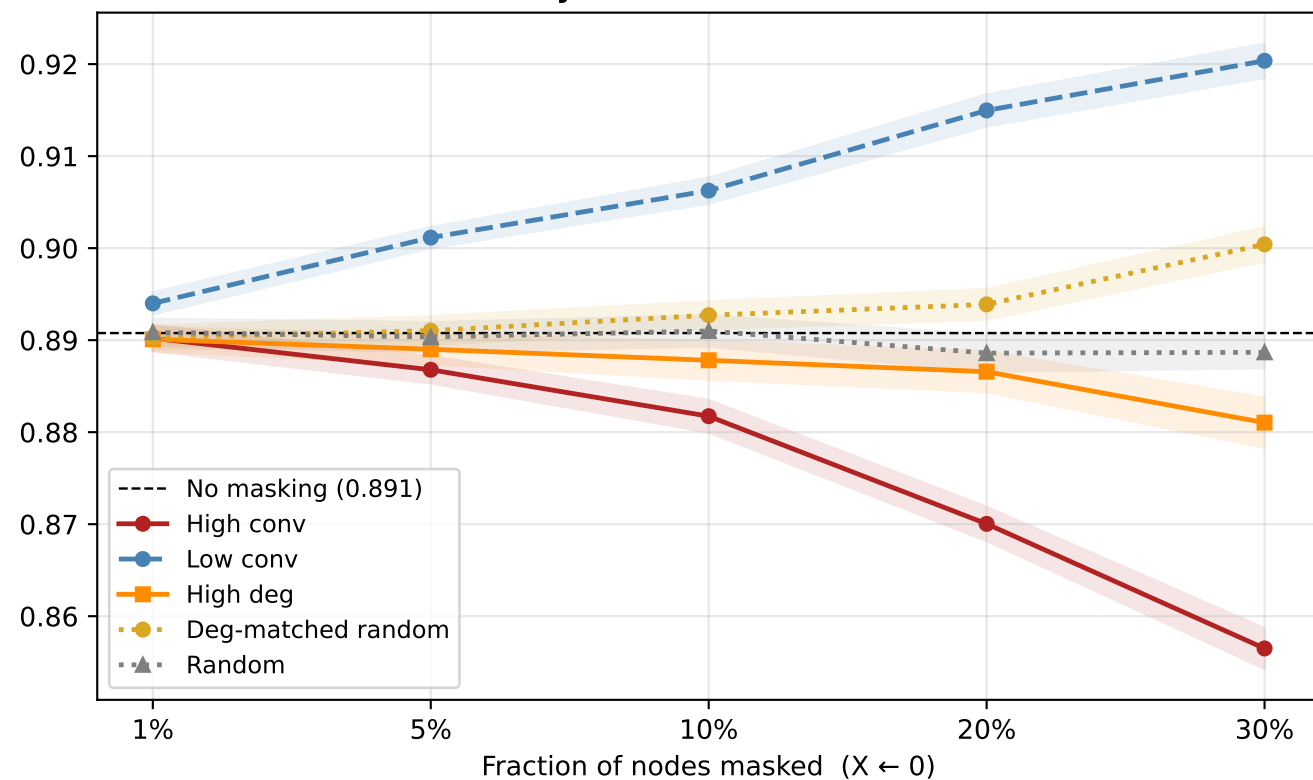
Accuracy on unmasked test nodes
