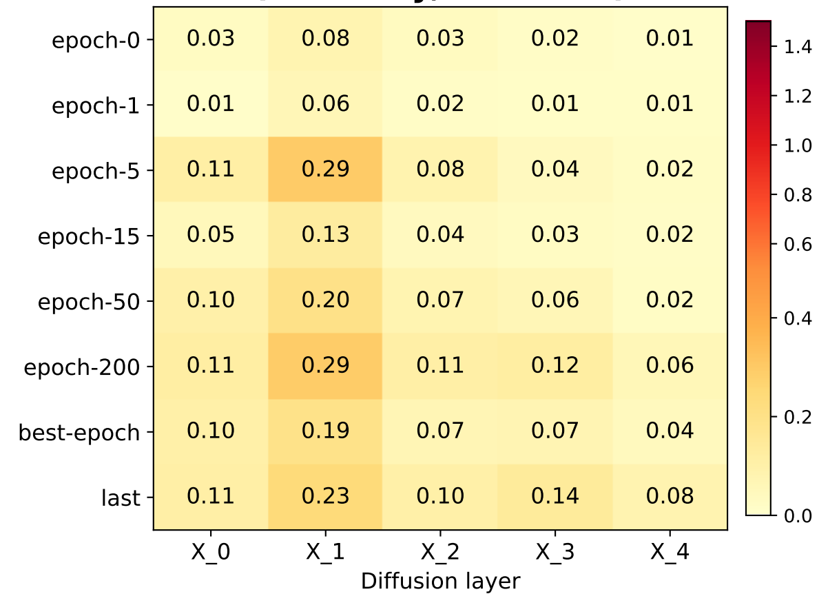
|Cohen's d| (accuracy, train set)
