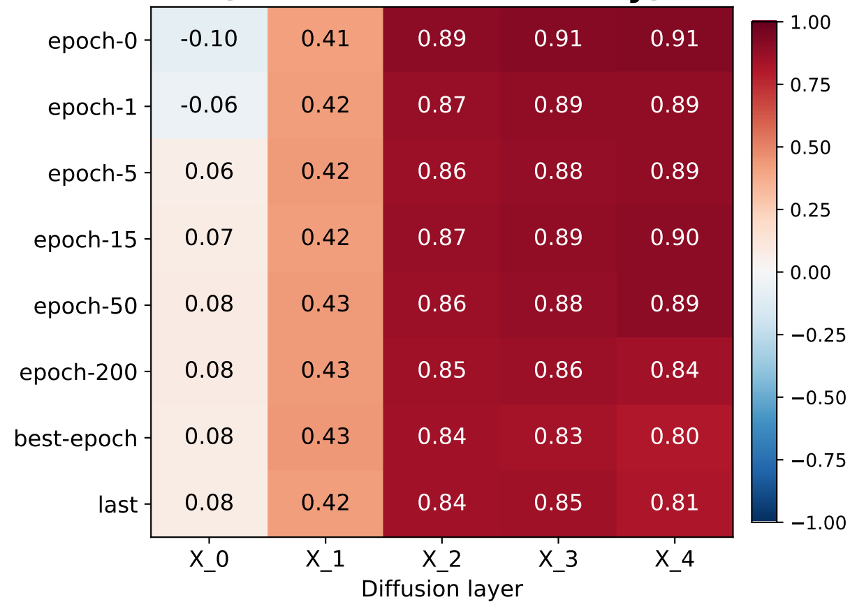
Spearman \rho (conviction vs saliency)
