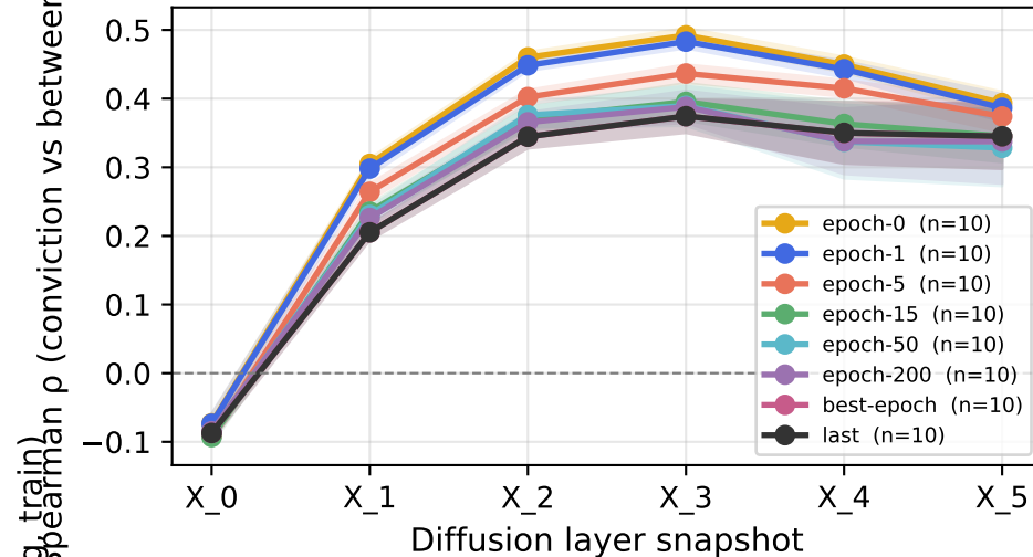
Conviction analysis over training — roman_empire (BundleSheaf, d=5, 5 layers)
