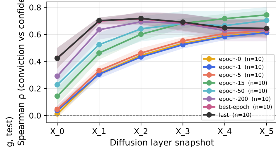
Conviction analysis over training — roman_empire (BundleSheaf, d=5, 5 layers)
