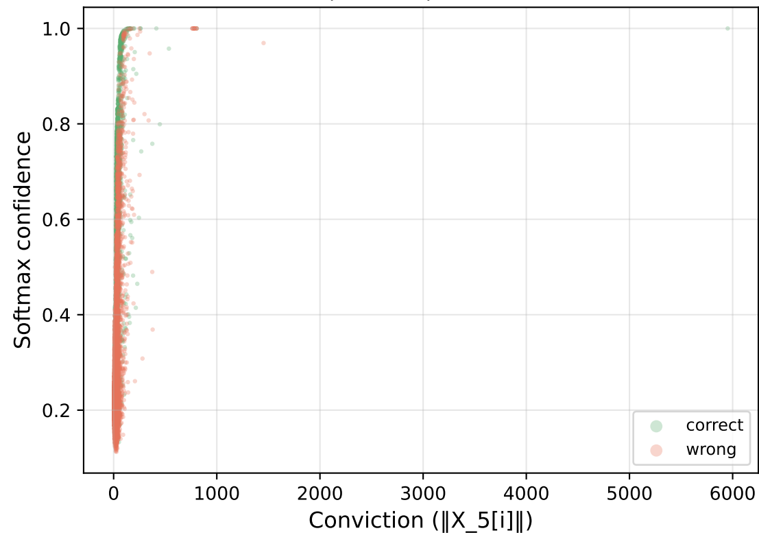
Conviction vs confidence (fold 0) Spearman \rho = 0.551
