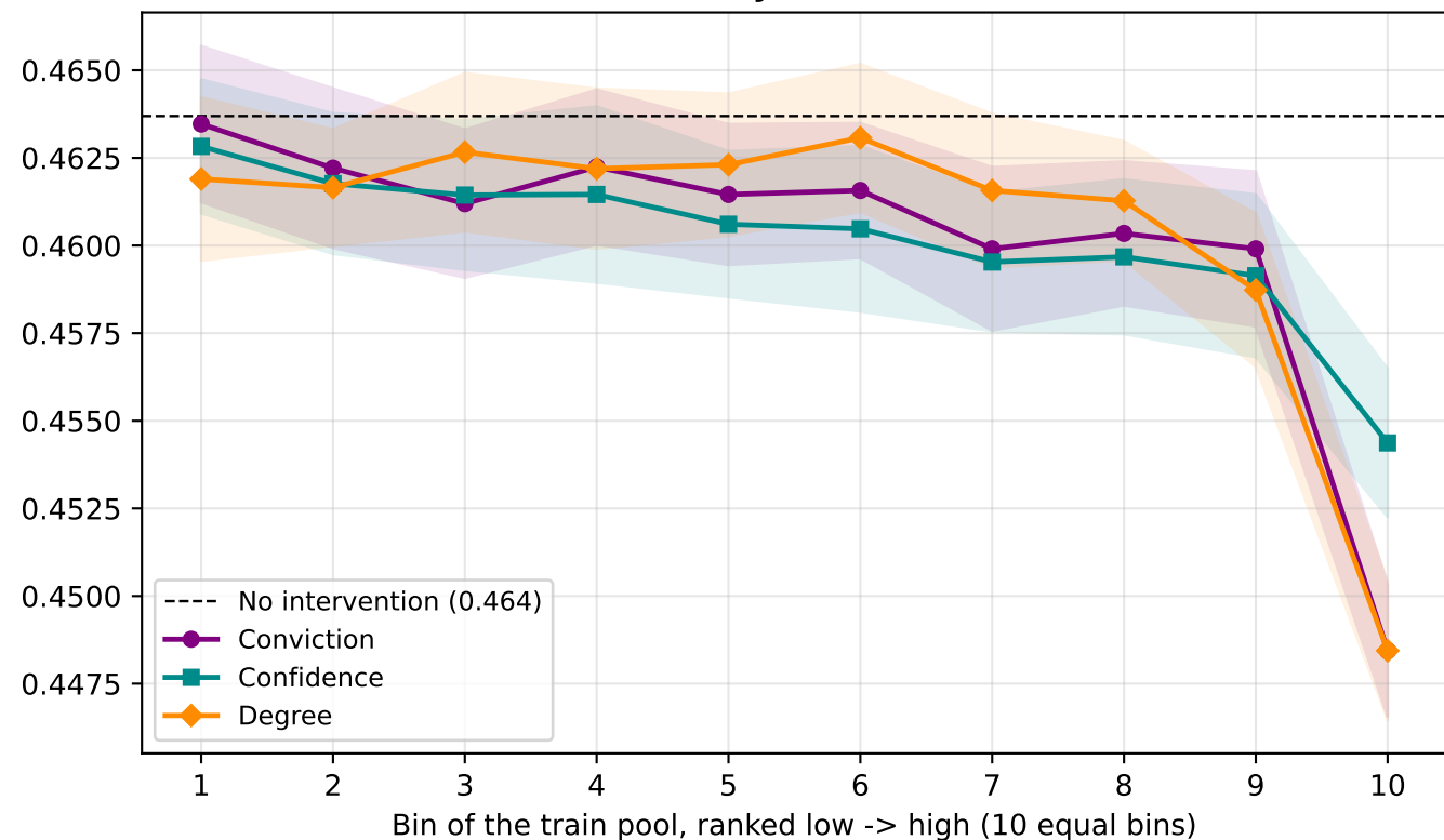
Accuracy on test set
