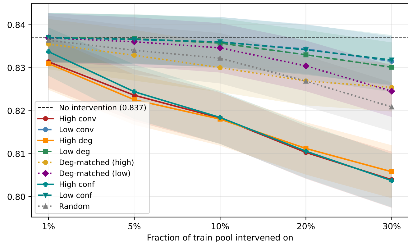
Mean confidence on test set
