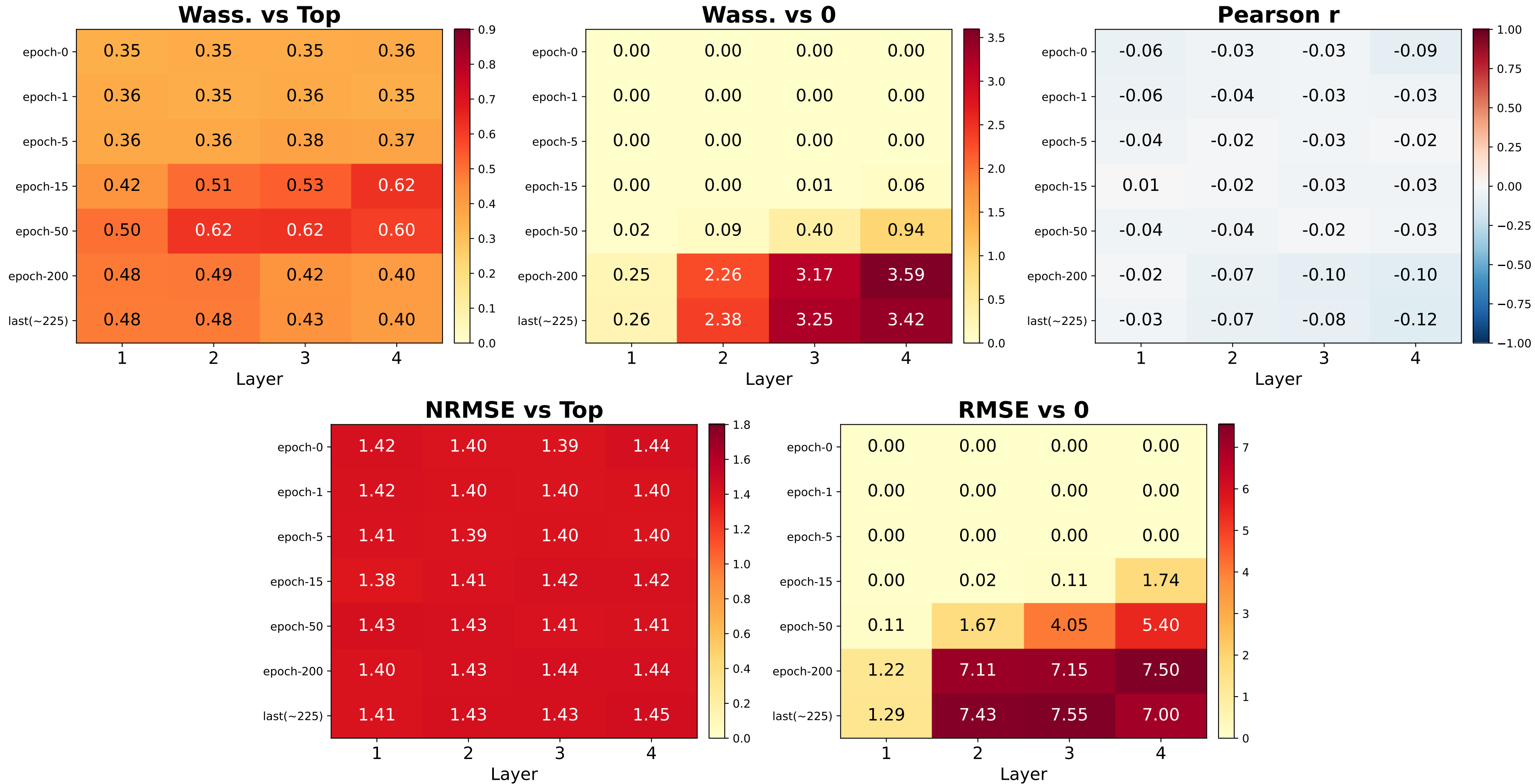
Forman Alignment Heatmap — citeseer (GeneralSheaf, d=5, 4L, norm=False) (values = mean across 5 eigenvalues, averaged over folds)
